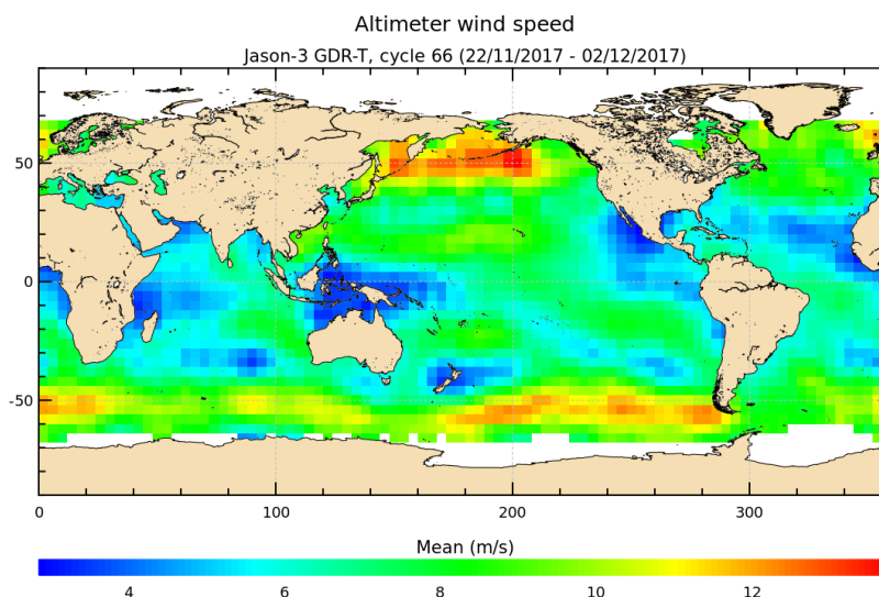
FIGURE 9 – Altimeter wind speed for cycle 066.
