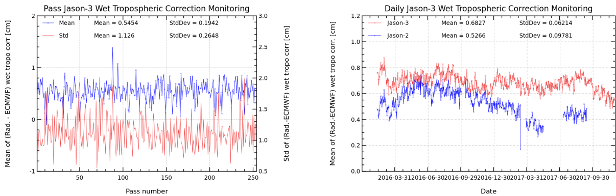
FIGURE 11 – Pass monitoring of wet troposphere differences between radiometer and ECMWF model for Jason-3 cycle 066 (left) and Jason-3 versus Jason-2 daily monitoring of wet troposphere differences between radiometer and ECMWF model (right).
