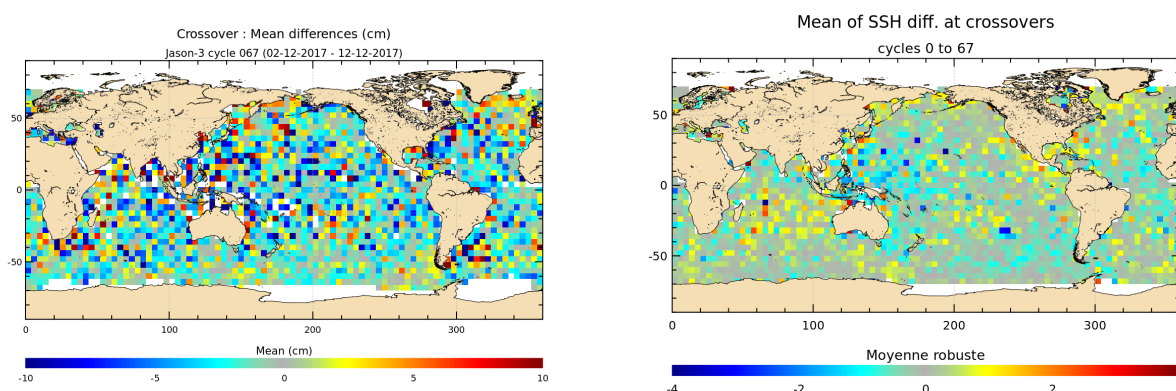
FIGURE 12 – Mean SSH at crossovers for cycle 067 (left) and over the whole Jason-3 period (right).
