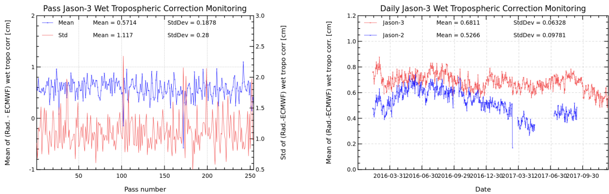
FIGURE 11 – Pass monitoring of wet troposphere differences between radiometer and ECMWF model for Jason-3 cycle 067 (left) and Jason-3 versus Jason-2 daily monitoring of wet troposphere differences between radiometer and ECMWF model (right).
