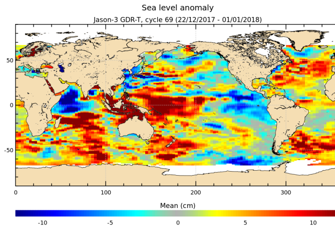
FIGURE 17 – Sea level anomaly relative to MSS for cycle 069.
