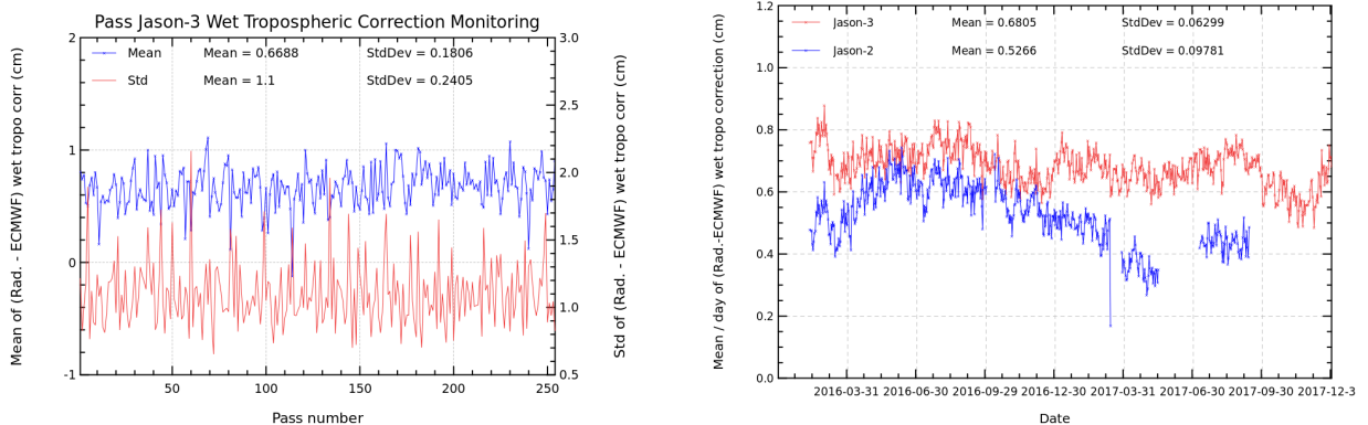
FIGURE 11 – Pass monitoring of wet troposphere differences between radiometer and ECMWF model for Jason-3 cycle 069 (left) and Jason-3 versus Jason-2 daily monitoring of wet troposphere differences between radiometer and ECMWF model (right).
