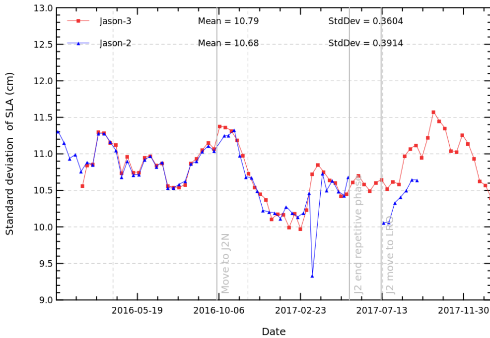
FIGURE 19 – Cyclic monitoring standard deviation of along track SLA for Jason-3 and Jason-2.
