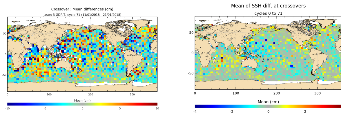
FIGURE 12 – Mean SSH at crossovers for cycle 071 (left) and over the whole Jason-3 period (right).
