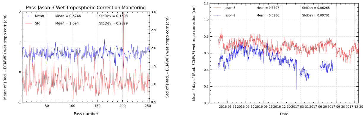
FIGURE 11 – Pass monitoring of wet troposphere differences between radiometer and ECMWF model for Jason-3 cycle 071 (left) and Jason-3 versus Jason-2 daily monitoring of wet troposphere differences between radiometer and ECMWF model (right).
