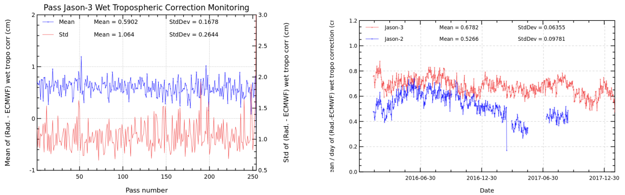
FIGURE 11 – Pass monitoring of wet troposphere differences between radiometer and ECMWF model for Jason-3 cycle 072 (left) and Jason-3 versus Jason-2 daily monitoring of wet troposphere differences between radiometer and ECMWF model (right).
