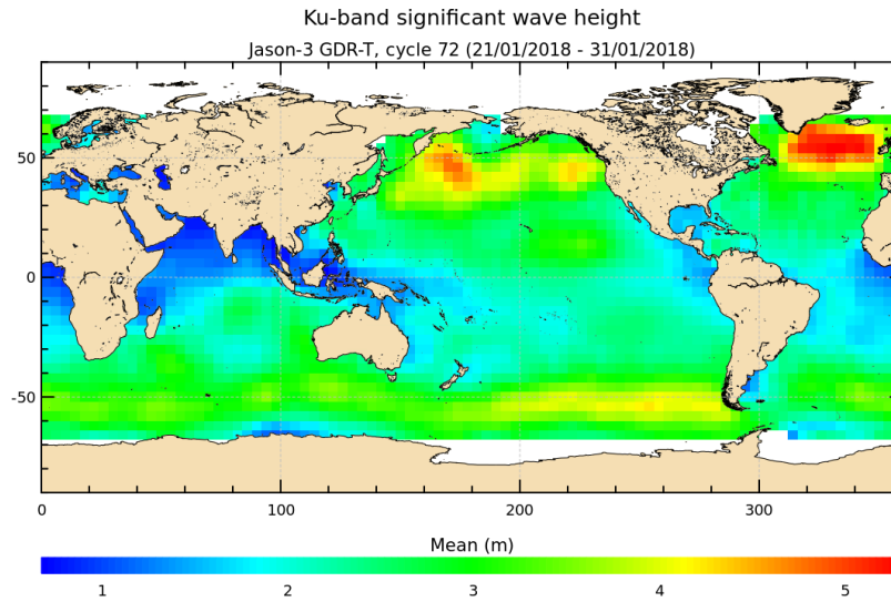
FIGURE 5 – Significant wave height for cycle 072.
