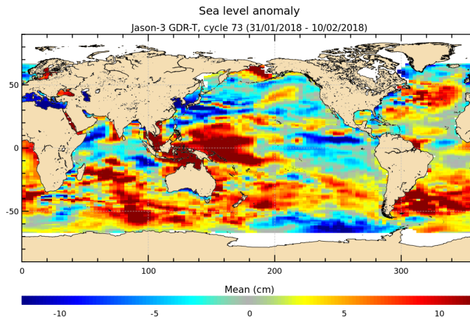
FIGURE 17 – Sea level anomaly relative to MSS for cycle 073.
