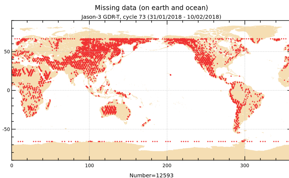
FIGURE 1 – Missing measurements for cycle 073.
