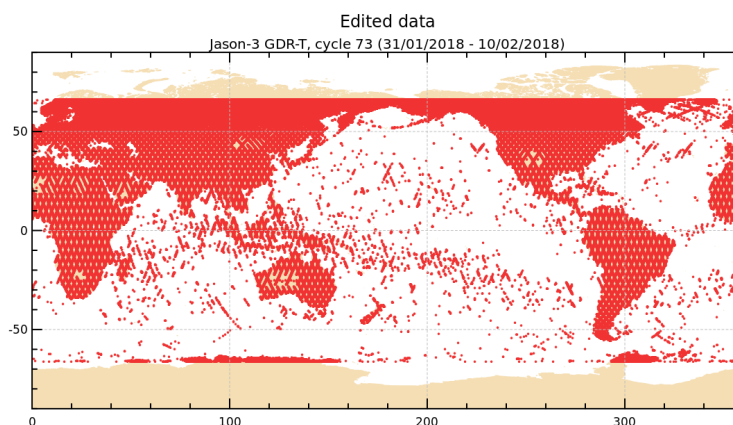
FIGURE 2 – Edited measurements for cycle 073.
