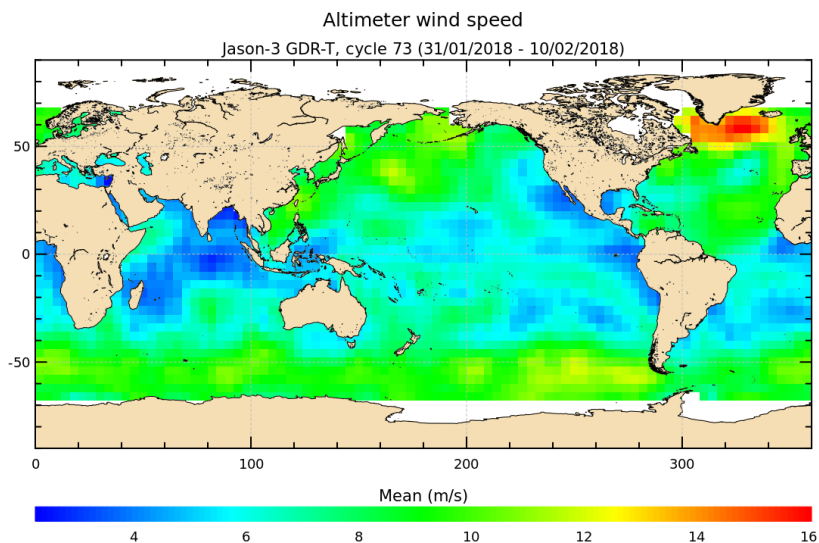
FIGURE 9 – Altimeter wind speed for cycle 073.
