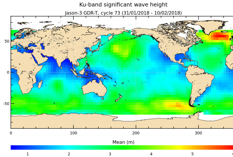
FIGURE 5 – Significant wave height for cycle 073.
