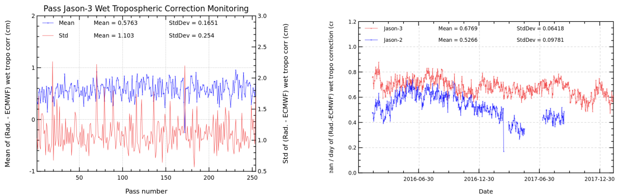
FIGURE 11 – Pass monitoring of wet troposphere differences between radiometer and ECMWF model for Jason-3 cycle 073 (left) and Jason-3 versus Jason-2 daily monitoring of wet troposphere differences between radiometer and ECMWF model (right).
