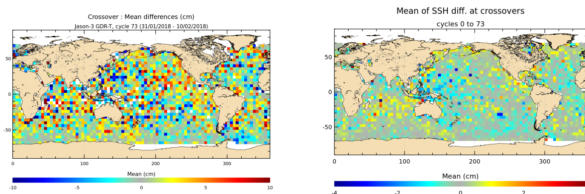
FIGURE 12 – Mean SSH at crossovers for cycle 073 (left) and over the whole Jason-3 period (right).
