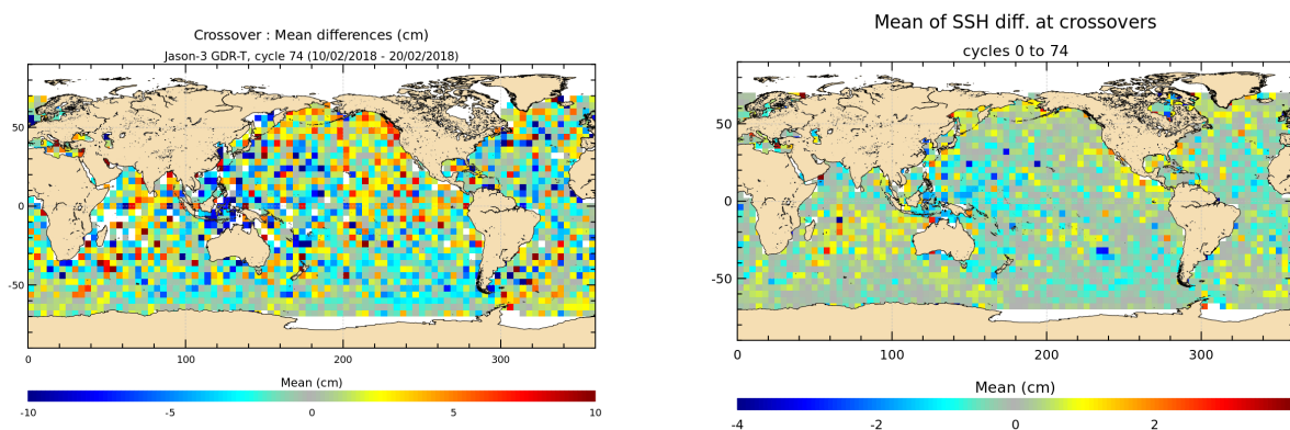
FIGURE 12 – Mean SSH at crossovers for cycle 074 (left) and over the whole Jason-3 period (right).
