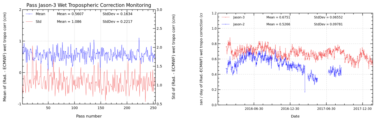
FIGURE 11 – Pass monitoring of wet troposphere differences between radiometer and ECMWF model for Jason-3 cycle 074 (left) and Jason-3 versus Jason-2 daily monitoring of wet troposphere differences between radiometer and ECMWF model (right).
