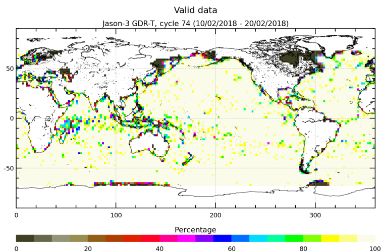
FIGURE 3 – Percentage of valid measurements for cycle 074.
