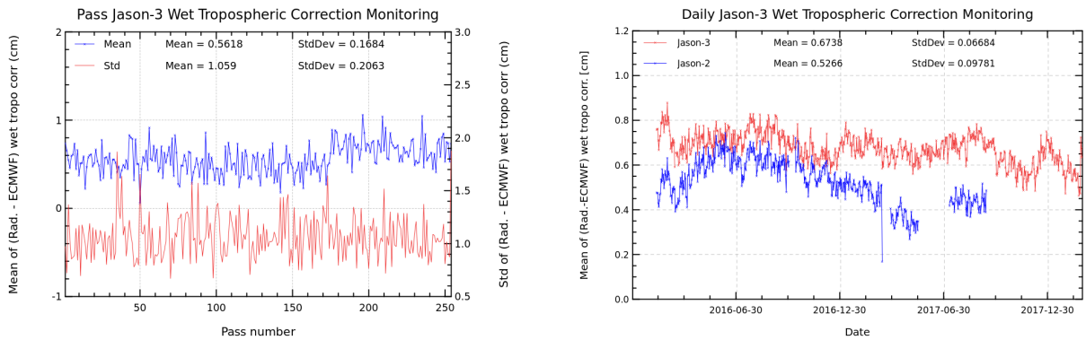
FIGURE 11 – Pass monitoring of wet troposphere differences between radiometer and ECMWF model for Jason-3 cycle 075 (left) and Jason-3 versus Jason-2 daily monitoring of wet troposphere differences between radiometer and ECMWF model (right).
