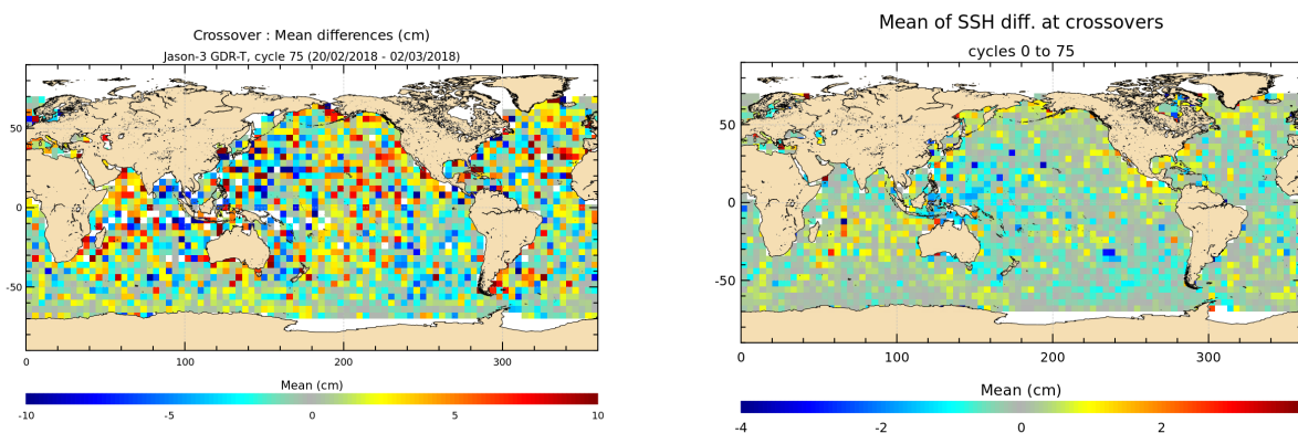
FIGURE 12 – Mean SSH at crossovers for cycle 075 (left) and over the whole Jason-3 period (right).
