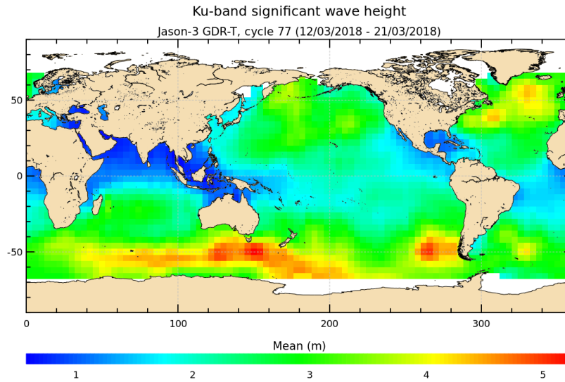
FIGURE 5 – Significant wave height for cycle 077.
