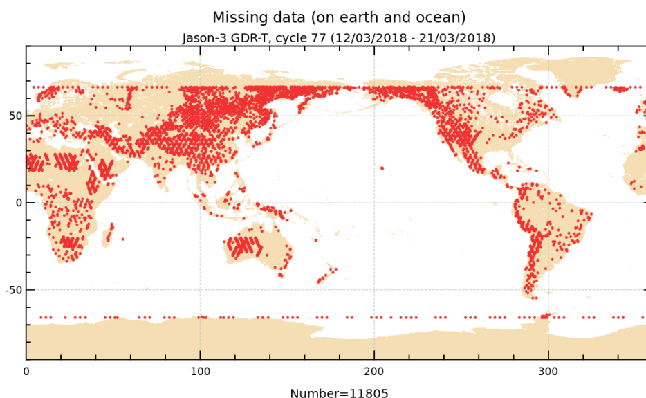
FIGURE 1 – Missing measurements for cycle 077.
