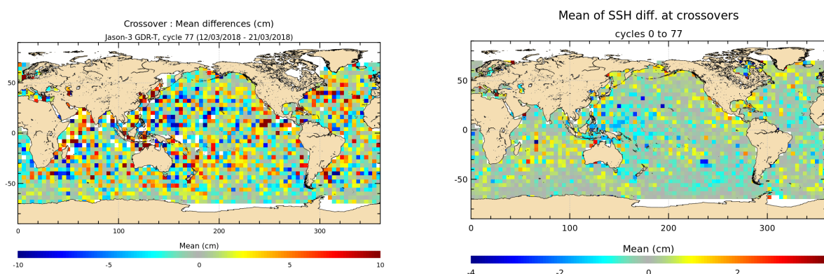
FIGURE 12 – Mean SSH at crossovers for cycle 077 (left) and over the whole Jason-3 period (right).
