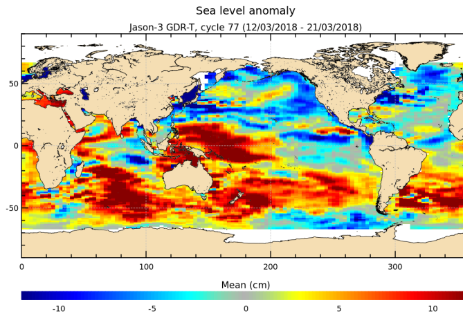
FIGURE 17 – Sea level anomaly relative to MSS for cycle 077.
