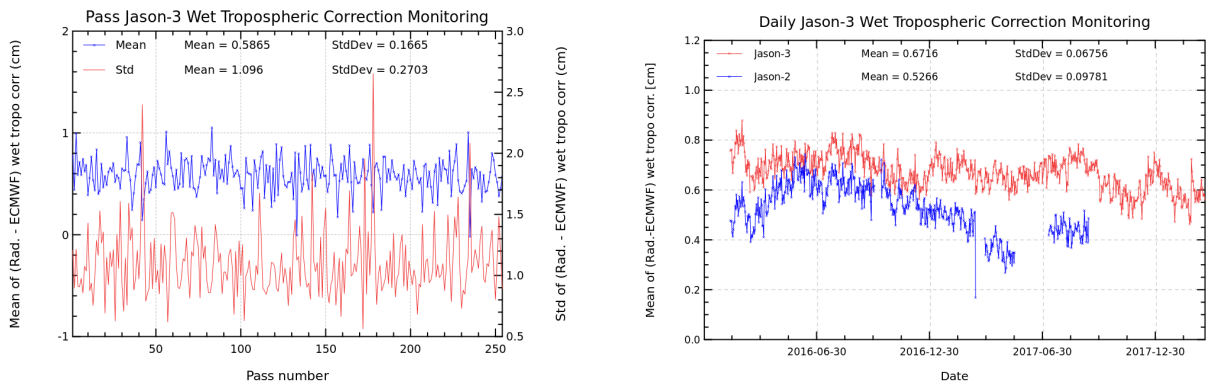
FIGURE 11 – Pass monitoring of wet troposphere differences between radiometer and ECMWF model for Jason-3 cycle 077 (left) and Jason-3 versus Jason-2 daily monitoring of wet troposphere differences between radiometer and ECMWF model (right).
