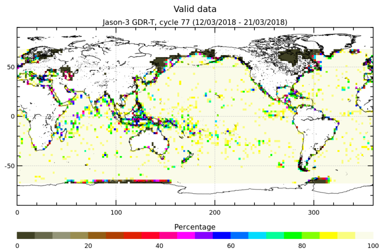
FIGURE 3 – Percentage of valid measurements for cycle 077.
