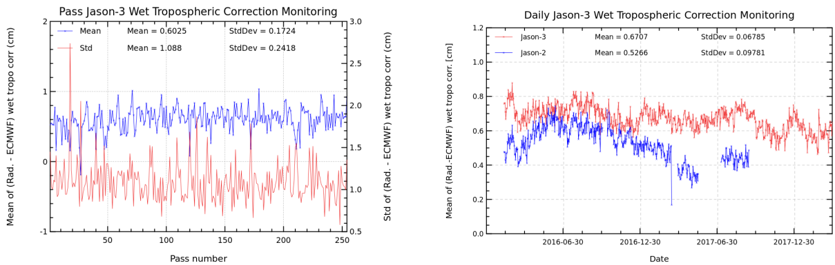
FIGURE 11 – Pass monitoring of wet troposphere differences between radiometer and ECMWF model for Jason-3 cycle 078 (left) and Jason-3 versus Jason-2 daily monitoring of wet troposphere differences between radiometer and ECMWF model (right).
