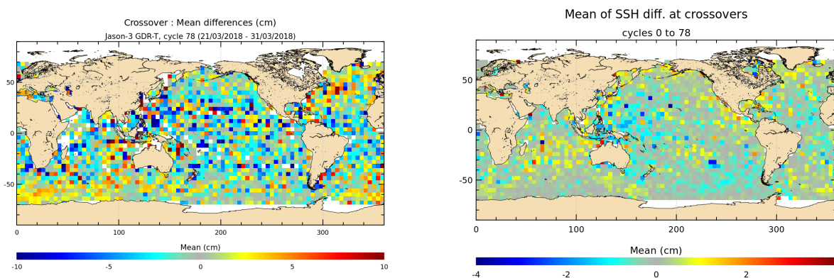
FIGURE 12 – Mean SSH at crossovers for cycle 078 (left) and over the whole Jason-3 period (right).
