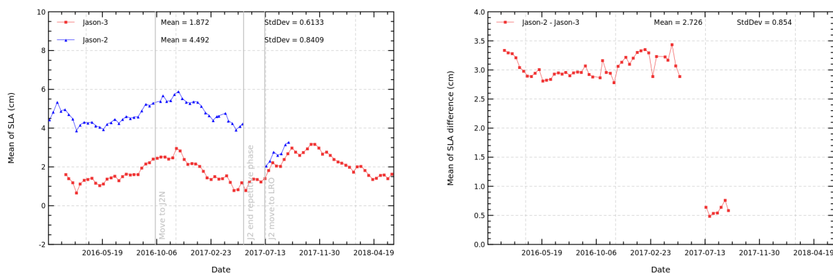
FIGURE 17 – Cyclic monitoring of mean SLA for Jason-3 and Jason-2 (left) and differences of (Jason-2 – Jason-3) mean SLA (right).
