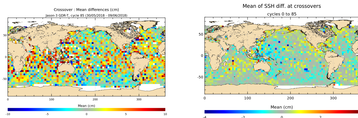
FIGURE 13 – Mean SSH at crossovers for cycle 085 (left) and over the whole Jason-3 period (right).
