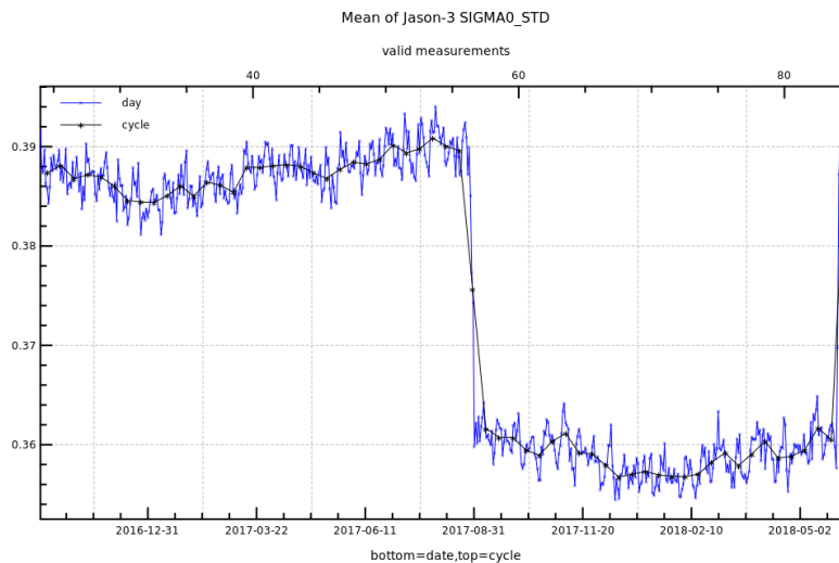
FIGURE 8 – Daily monitoring of Ku-band backscattering coefficient for Jason-3.
