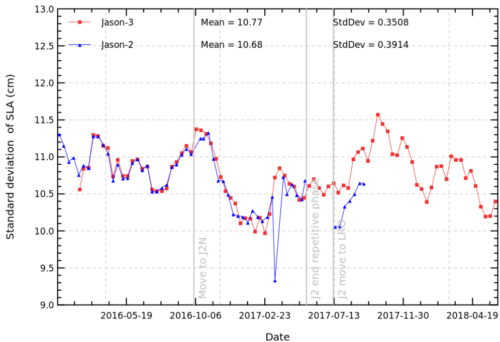
FIGURE 20 – Cyclic monitoring standard deviation of along track SLA for Jason-3 and Jason-2.
