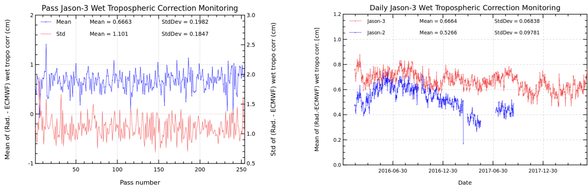
FIGURE 12 – Pass monitoring of wet troposphere differences between radiometer and ECMWF model for Jason-3 cycle 085 (left) and Jason-3 versus Jason-2 daily monitoring of wet troposphere differences between radiometer and ECMWF model (right).
