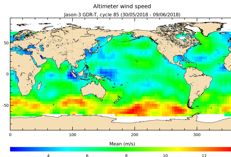
FIGURE 10 – Altimeter wind speed for cycle 085.
