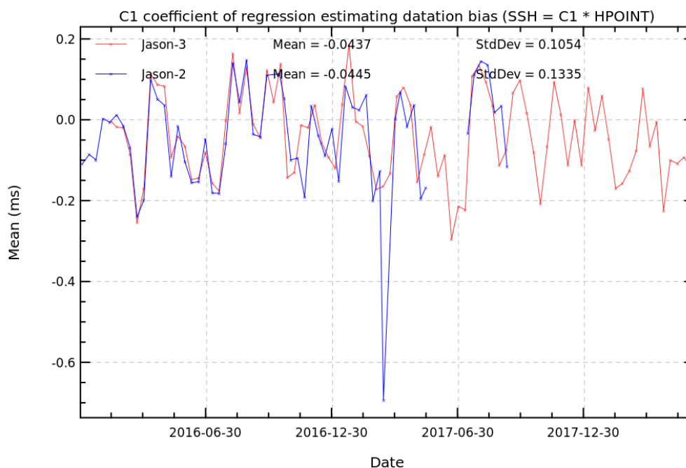
FIGURE 16 – Cyclic monitoring of pseudo time tag bias for Jason-3 and Jason-2.
