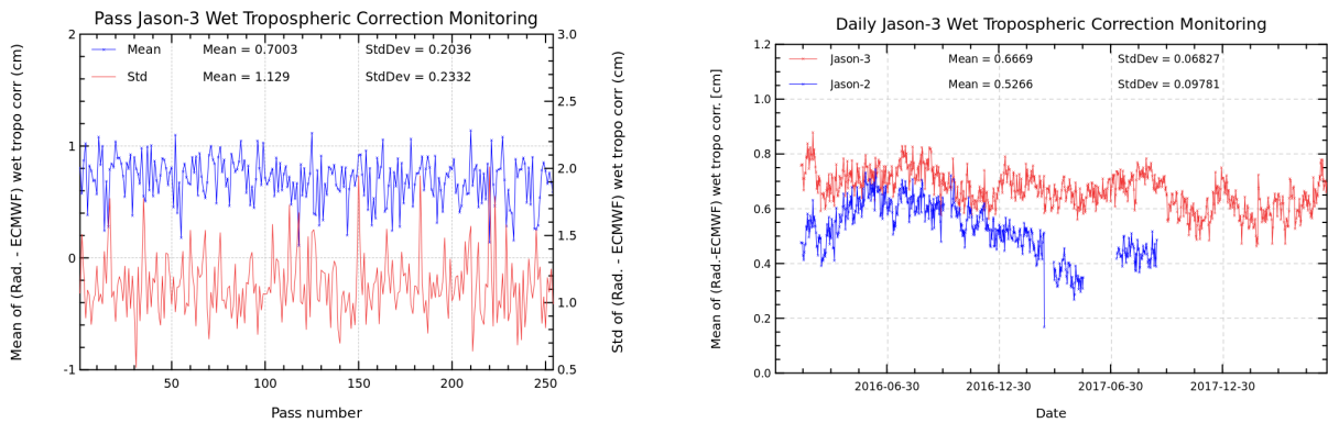
FIGURE 11 – Pass monitoring of wet troposphere differences between radiometer and ECMWF model for Jason-3 cycle 086 (left) and Jason-3 versus Jason-2 daily monitoring of wet troposphere differences between radiometer and ECMWF model (right).
