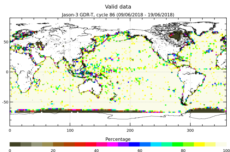
FIGURE 3 – Percentage of valid measurements for cycle 086.
