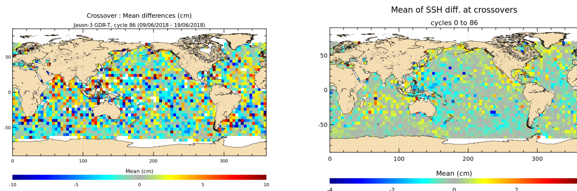
FIGURE 12 – Mean SSH at crossovers for cycle 086 (left) and over the whole Jason-3 period (right).
