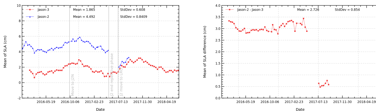
FIGURE 17 – Cyclic monitoring of mean SLA for Jason-3 and Jason-2 (left) and differences of (Jason-2 – Jason-3) mean SLA (right).
