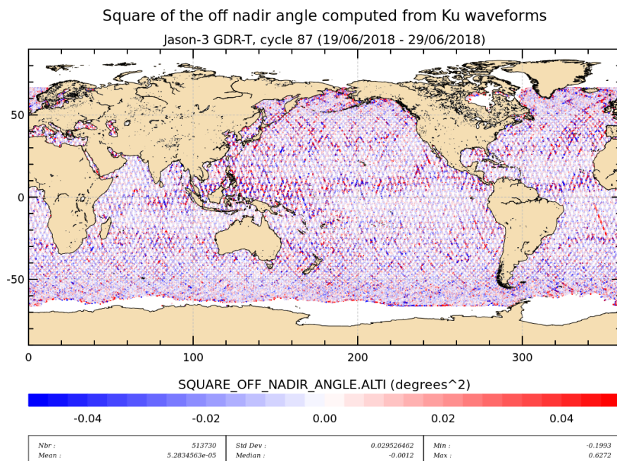
FIGURE 4 – Apparent squared mispointing from waveforms for cycle 087.
