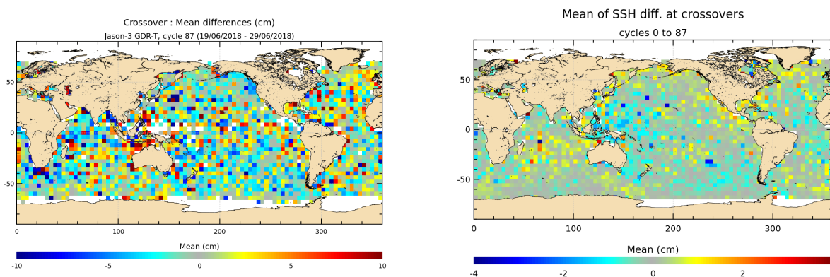
FIGURE 13 – Mean SSH at crossovers for cycle 087 (left) and over the whole Jason-3 period (right).
