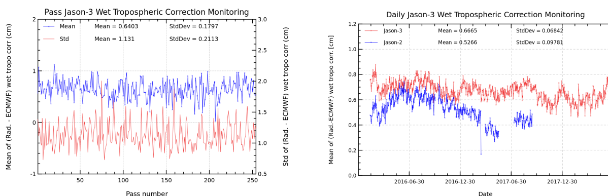
FIGURE 12 – Pass monitoring of wet troposphere differences between radiometer and ECMWF model for Jason-3 cycle 087 (left) and Jason-3 versus Jason-2 daily monitoring of wet troposphere differences between radiometer and ECMWF model (right).
