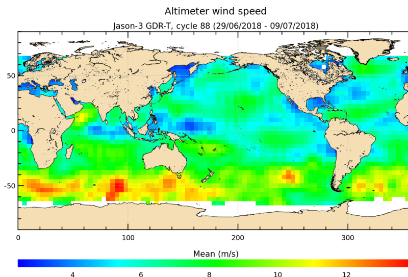
FIGURE 9 – Altimeter wind speed for cycle 088.
