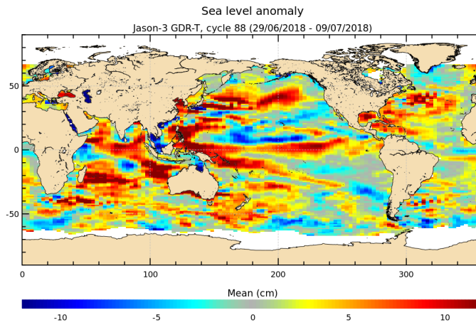
FIGURE 17 – Sea level anomaly relative to MSS for cycle 088.
