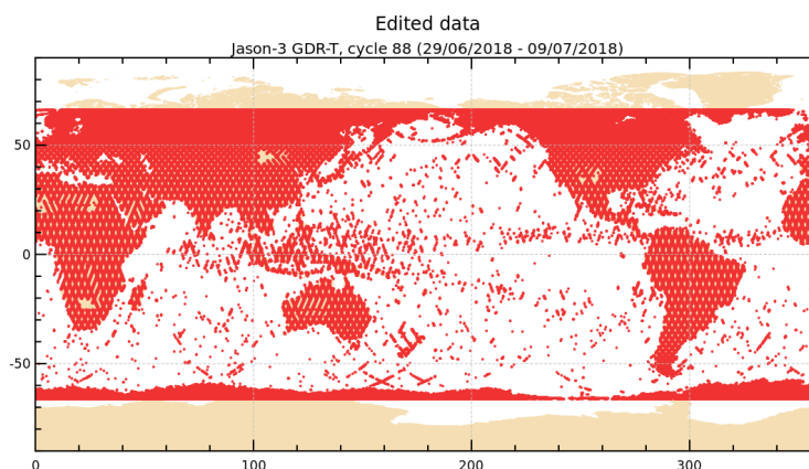
FIGURE 2 – Edited measurements for cycle 088.
