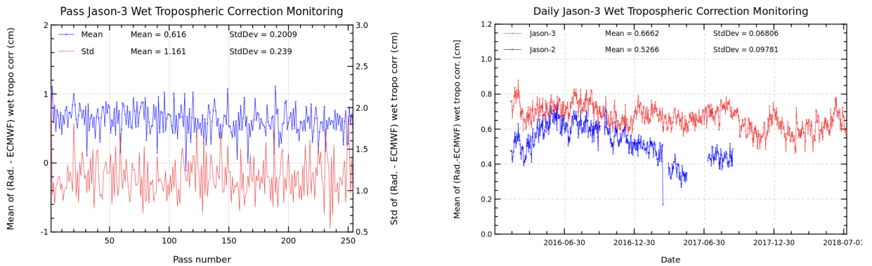
FIGURE 11 – Pass monitoring of wet troposphere differences between radiometer and ECMWF model for Jason-3 cycle 088 (left) and Jason-3 versus Jason-2 daily monitoring of wet troposphere differences between radiometer and ECMWF model (right).
