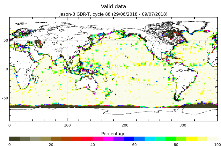
FIGURE 3 – Percentage of valid measurements for cycle 088.
