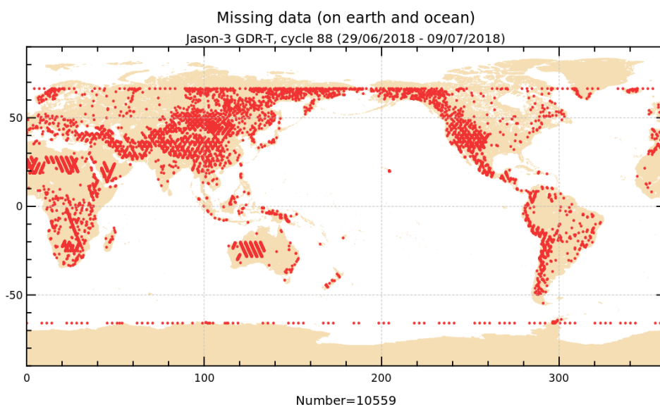
FIGURE 1 – Missing measurements for cycle 088.
