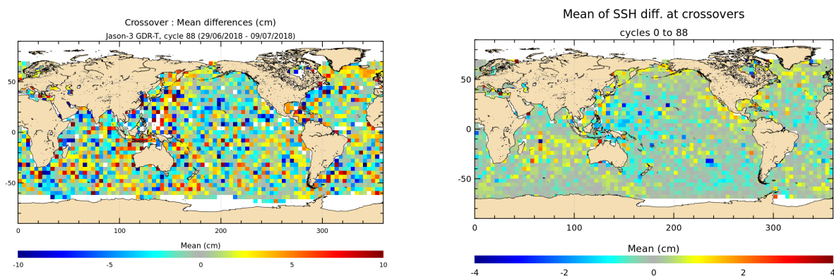
FIGURE 12 – Mean SSH at crossovers for cycle 088 (left) and over the whole Jason-3 period (right).
