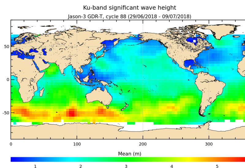
FIGURE 5 – Significant wave height for cycle 088.
