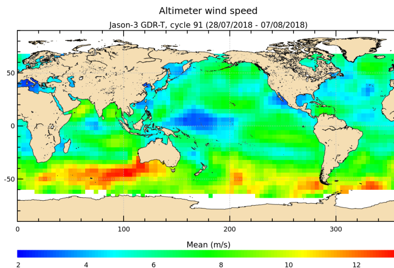
FIGURE 9 – Altimeter wind speed for cycle 091.
