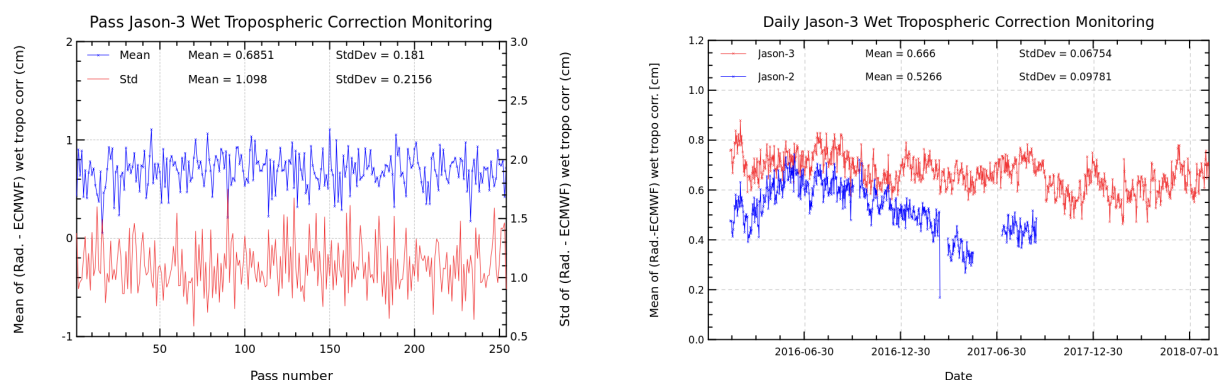
FIGURE 11 – Pass monitoring of wet troposphere differences between radiometer and ECMWF model for Jason-3 cycle 091 (left) and Jason-3 versus Jason-2 daily monitoring of wet troposphere differences between radiometer and ECMWF model (right).
