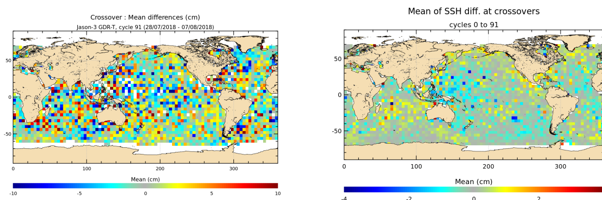
FIGURE 12 – Mean SSH at crossovers for cycle 091 (left) and over the whole Jason-3 period (right).
