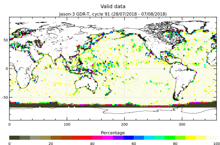
FIGURE 3 – Percentage of valid measurements for cycle 091.
