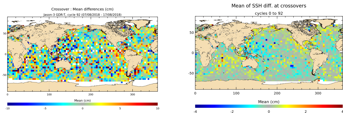
FIGURE 12 – Mean SSH at crossovers for cycle 092 (left) and over the whole Jason-3 period (right).
