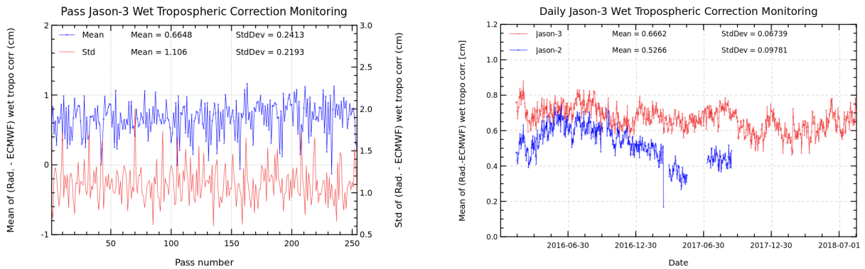
FIGURE 11 – Pass monitoring of wet troposphere differences between radiometer and ECMWF model for Jason-3 cycle 092 (left) and Jason-3 versus Jason-2 daily monitoring of wet troposphere differences between radiometer and ECMWF model (right).
