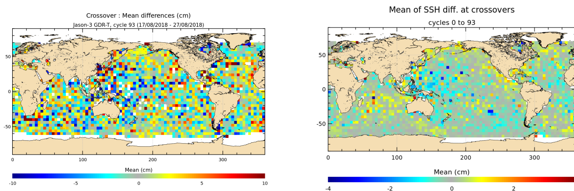
FIGURE 12 – Mean SSH at crossovers for cycle 093 (left) and over the whole Jason-3 period (right).
