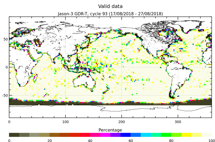
FIGURE 3 – Percentage of valid measurements for cycle 093.
