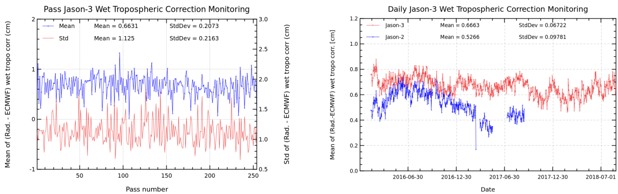
FIGURE 11 – Pass monitoring of wet troposphere differences between radiometer and ECMWF model for Jason-3 cycle 093 (left) and Jason-3 versus Jason-2 daily monitoring of wet troposphere differences between radiometer and ECMWF model (right).
