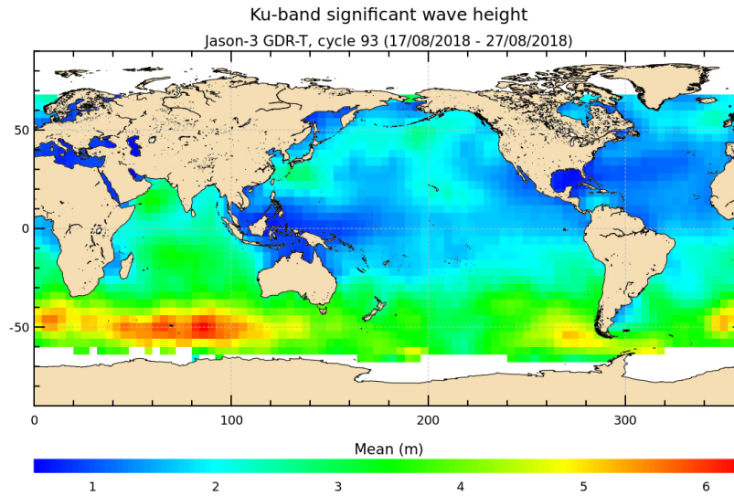
FIGURE 5 – Significant wave height for cycle 093.
