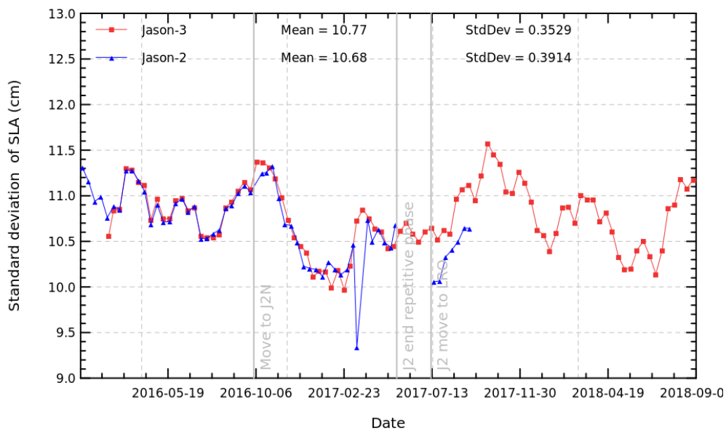
FIGURE 19 – Cyclic monitoring standard deviation of along track SLA for Jason-3 and Jason-2.
