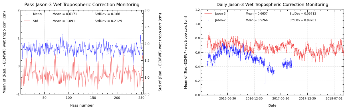
FIGURE 11 – Pass monitoring of wet troposphere differences between radiometer and ECMWF model for Jason-3 cycle 094 (left) and Jason-3 versus Jason-2 daily monitoring of wet troposphere differences between radiometer and ECMWF model (right).
