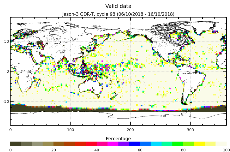
FIGURE 3 – Percentage of valid measurements for cycle 098.
