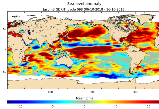
FIGURE 17 – Sea level anomaly relative to MSS for cycle 098.
