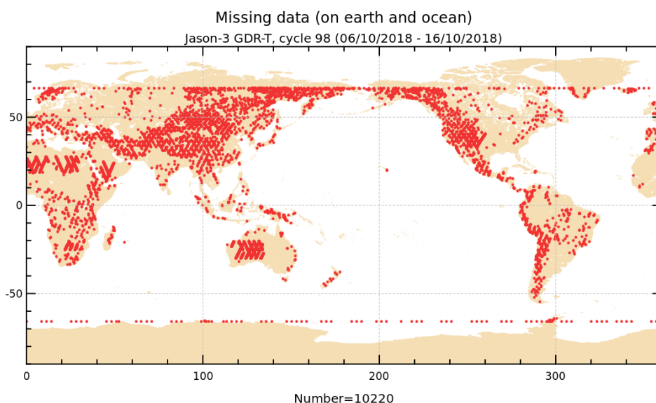
FIGURE 1 – Missing measurements for cycle 098.
