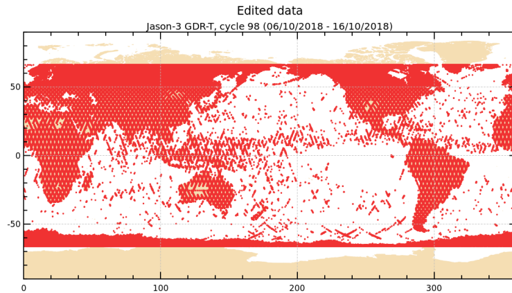
FIGURE 2 – Edited measurements for cycle 098.
