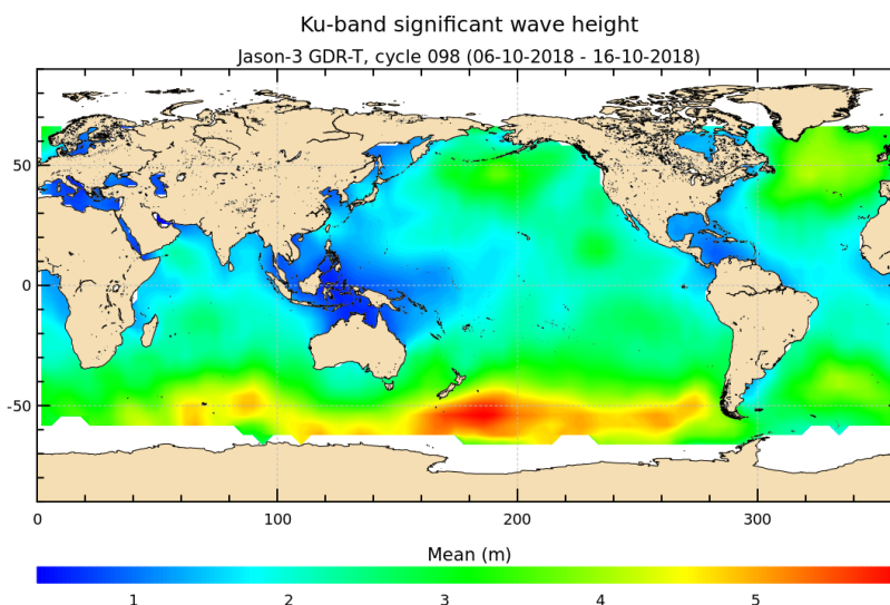
FIGURE 5 – Significant wave height for cycle 098.
