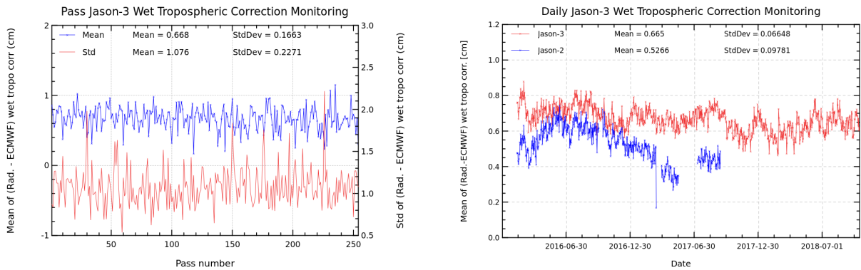
FIGURE 11 – Pass monitoring of wet troposphere differences between radiometer and ECMWF model for Jason-3 cycle 098 (left) and Jason-3 versus Jason-2 daily monitoring of wet troposphere differences between radiometer and ECMWF model (right).
