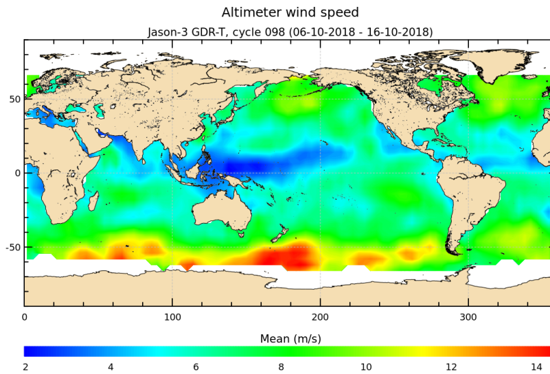
FIGURE 9 – Altimeter wind speed for cycle 098.
