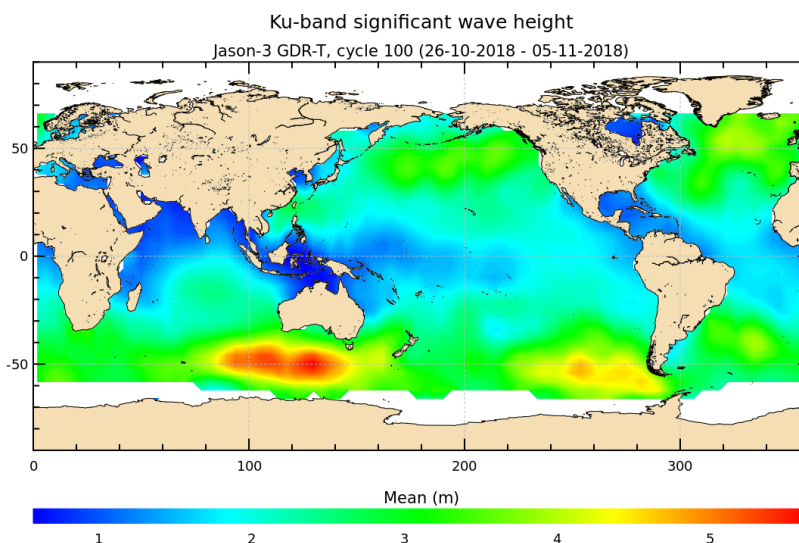
FIGURE 5 – Significant wave height for cycle 100.
