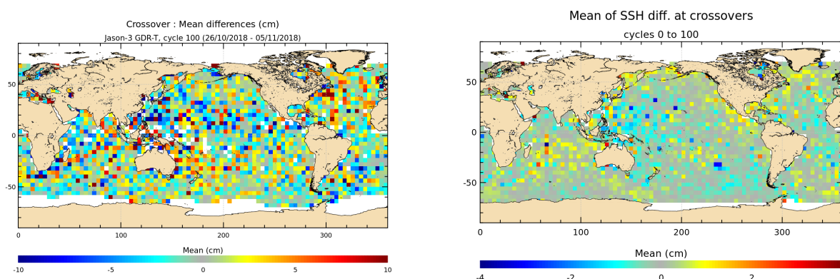
FIGURE 12 – Mean SSH at crossovers for cycle 100 (left) and over the whole Jason-3 period (right).
