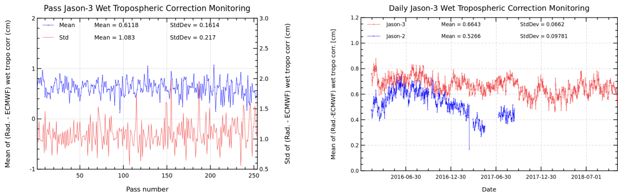
FIGURE 11 – Pass monitoring of wet troposphere differences between radiometer and ECMWF model for Jason-3 cycle 100 (left) and Jason-3 versus Jason-2 daily monitoring of wet troposphere differences between radiometer and ECMWF model (right).
