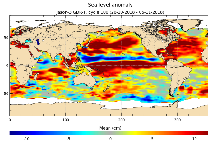
FIGURE 17 – Sea level anomaly relative to MSS for cycle 100.
