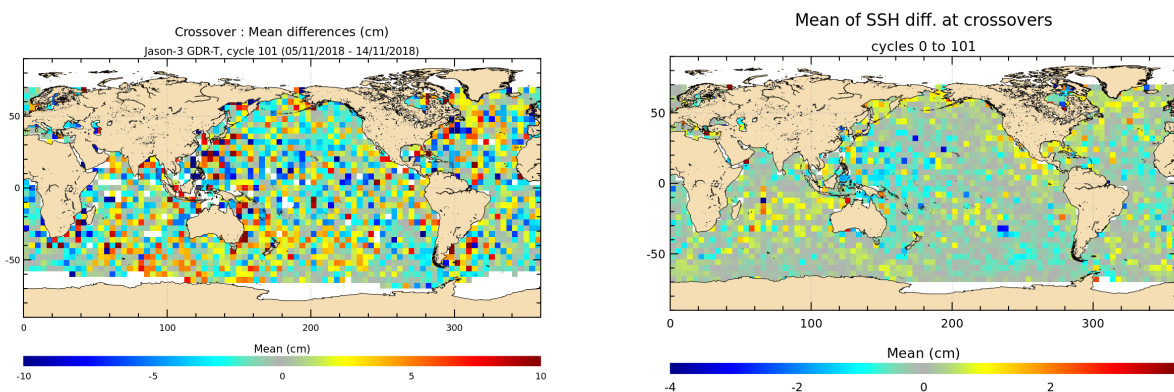
FIGURE 12 – Mean SSH at crossovers for cycle 101 (left) and over the whole Jason-3 period (right).
