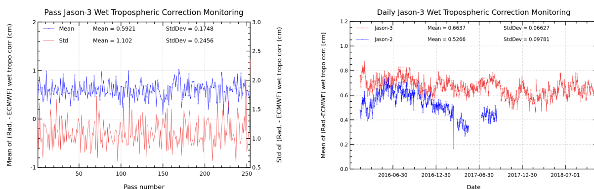
FIGURE 11 – Pass monitoring of wet troposphere differences between radiometer and ECMWF model for Jason-3 cycle 101 (left) and Jason-3 versus Jason-2 daily monitoring of wet troposphere differences between radiometer and ECMWF model (right).
