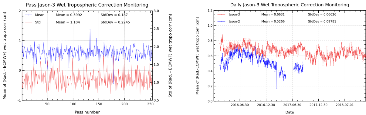
FIGURE 11 – Pass monitoring of wet troposphere differences between radiometer and ECMWF model for Jason-3 cycle 102 (left) and Jason-3 versus Jason-2 daily monitoring of wet troposphere differences between radiometer and ECMWF model (right).
