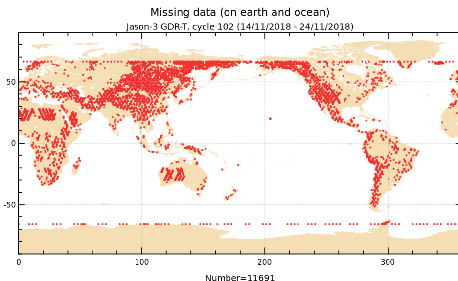
FIGURE 1 – Missing measurements for cycle 102.
