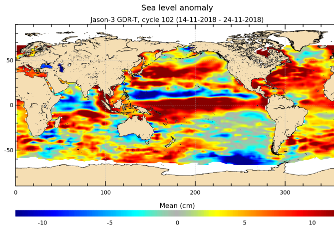
FIGURE 17 – Sea level anomaly relative to MSS for cycle 102.
