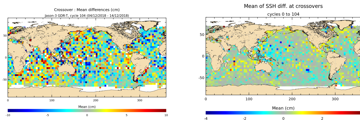
FIGURE 12 – Mean SSH at crossovers for cycle 104 (left) and over the whole Jason-3 period (right).
