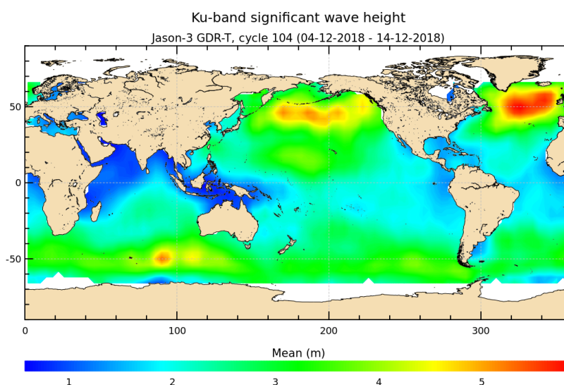
FIGURE 5 – Significant wave height for cycle 104.
