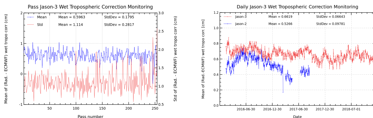
FIGURE 11 – Pass monitoring of wet troposphere differences between radiometer and ECMWF model for Jason-3 cycle 104 (left) and Jason-3 versus Jason-2 daily monitoring of wet troposphere differences between radiometer and ECMWF model (right).
