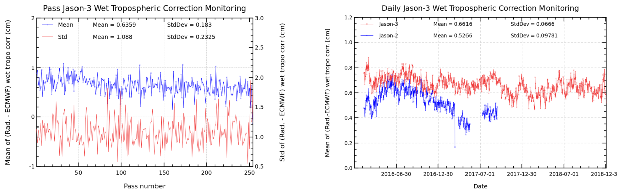
FIGURE 11 – Pass monitoring of wet troposphere differences between radiometer and ECMWF model for Jason-3 cycle 106 (left) and Jason-3 versus Jason-2 daily monitoring of wet troposphere differences between radiometer and ECMWF model (right).
