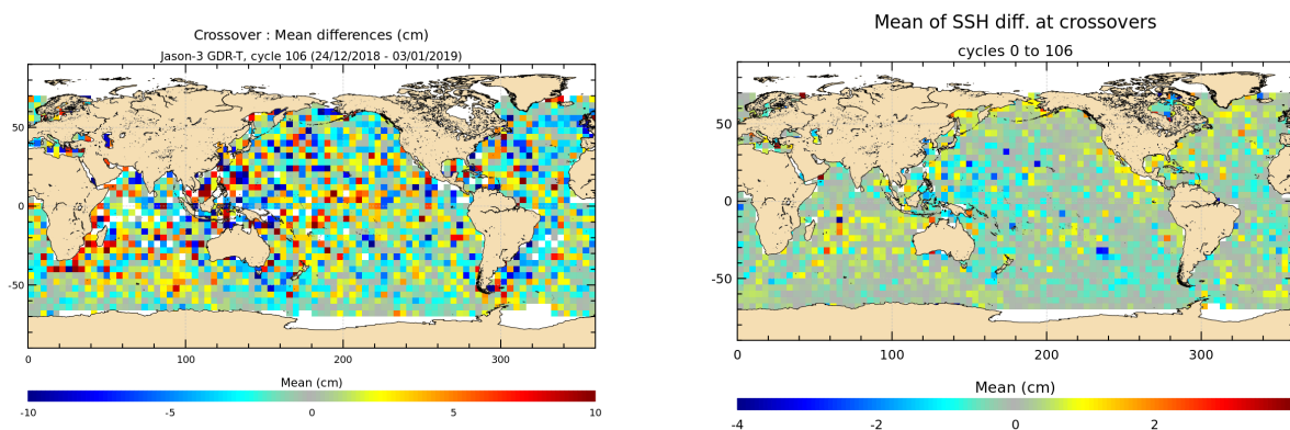
FIGURE 12 – Mean SSH at crossovers for cycle 106 (left) and over the whole Jason-3 period (right).
