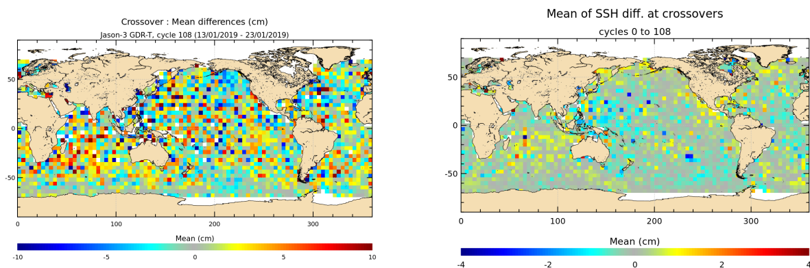
FIGURE 12 – Mean SSH at crossovers for cycle 108 (left) and over the whole Jason-3 period (right).
