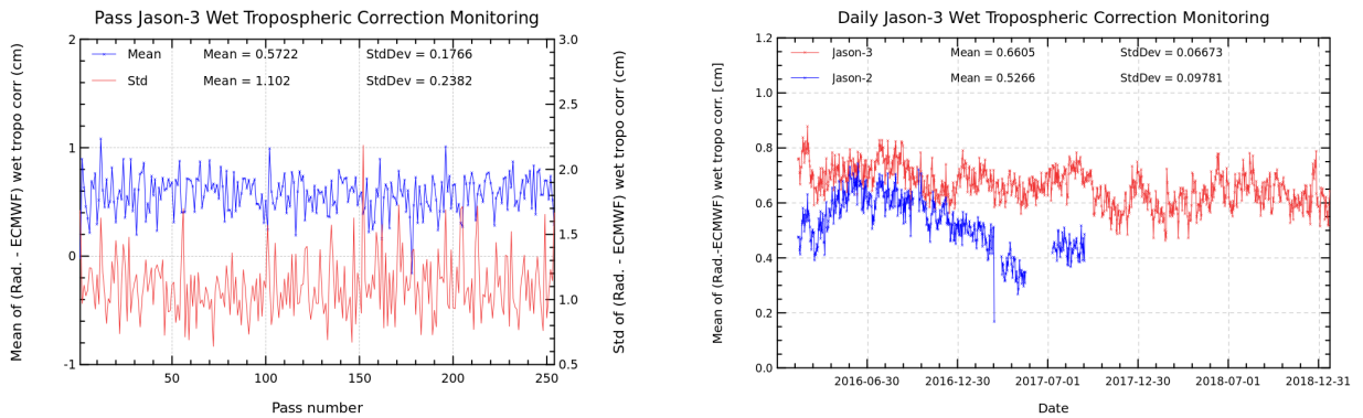
FIGURE 11 – Pass monitoring of wet troposphere differences between radiometer and ECMWF model for Jason-3 cycle 108 (left) and Jason-3 versus Jason-2 daily monitoring of wet troposphere differences between radiometer and ECMWF model (right).
