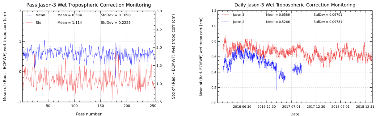
FIGURE 11 – Pass monitoring of wet troposphere differences between radiometer and ECMWF model for Jason-3 cycle 111 (left) and Jason-3 versus Jason-2 daily monitoring of wet troposphere differences between radiometer and ECMWF model (right).
