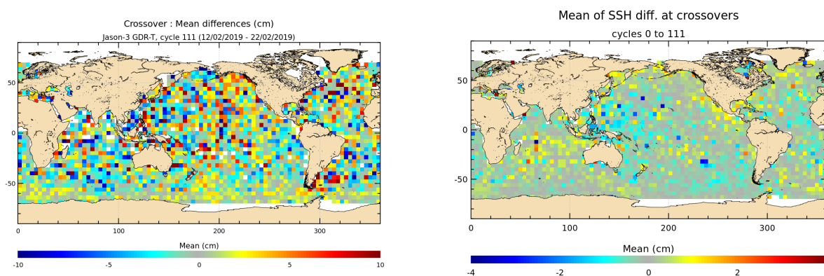
FIGURE 12 – Mean SSH at crossovers for cycle 111 (left) and over the whole Jason-3 period (right).
