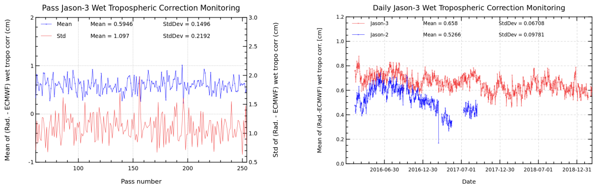
FIGURE 11 – Pass monitoring of wet troposphere differences between radiometer and ECMWF model for Jason-3 cycle 113 (left) and Jason-3 versus Jason-2 daily monitoring of wet troposphere differences between radiometer and ECMWF model (right).
