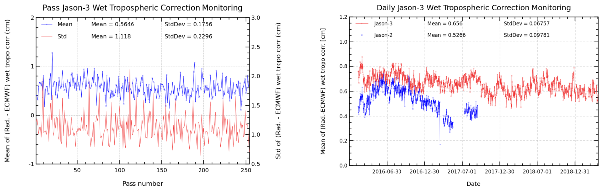
FIGURE 11 – Pass monitoring of wet troposphere differences between radiometer and ECMWF model for Jason-3 cycle 117 (left) and Jason-3 versus Jason-2 daily monitoring of wet troposphere differences between radiometer and ECMWF model (right).
