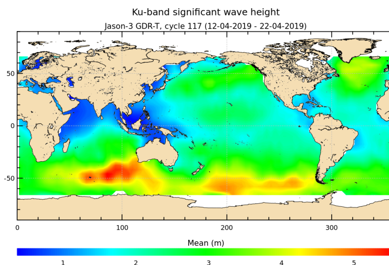
FIGURE 5 – Significant wave height for cycle 117.
