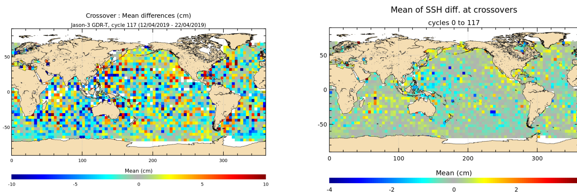
FIGURE 12 – Mean SSH at crossovers for cycle 117 (left) and over the whole Jason-3 period (right).
