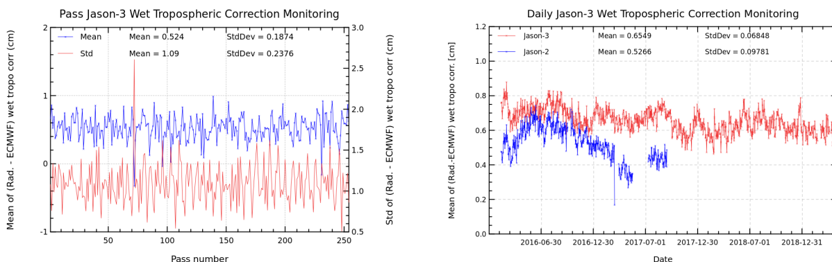
FIGURE 11 – Pass monitoring of wet troposphere differences between radiometer and ECMWF model for Jason-3 cycle 118 (left) and Jason-3 versus Jason-2 daily monitoring of wet troposphere differences between radiometer and ECMWF model (right).
