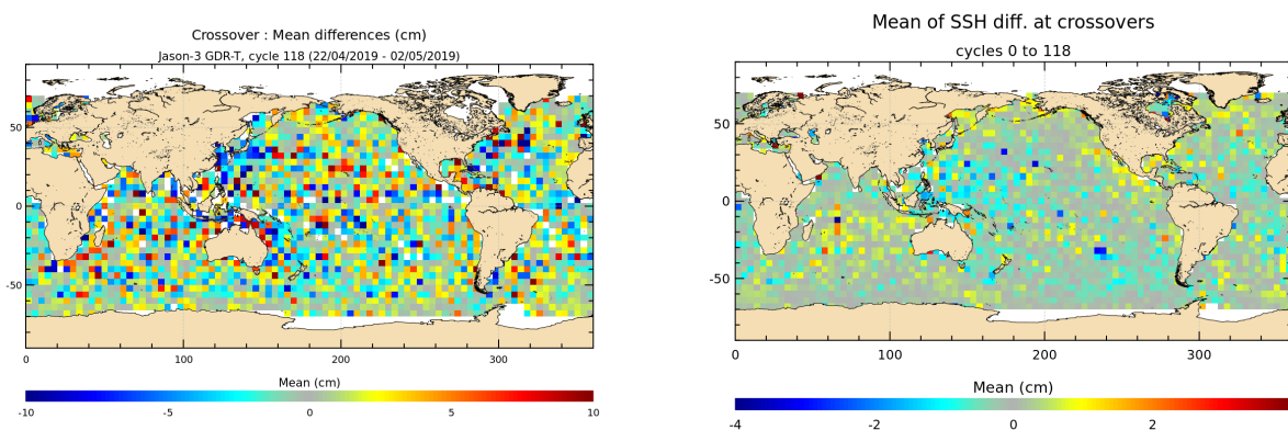
FIGURE 12 – Mean SSH at crossovers for cycle 118 (left) and over the whole Jason-3 period (right).
