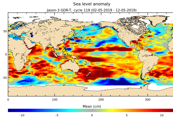
FIGURE 17 – Sea level anomaly relative to MSS for cycle 119.
