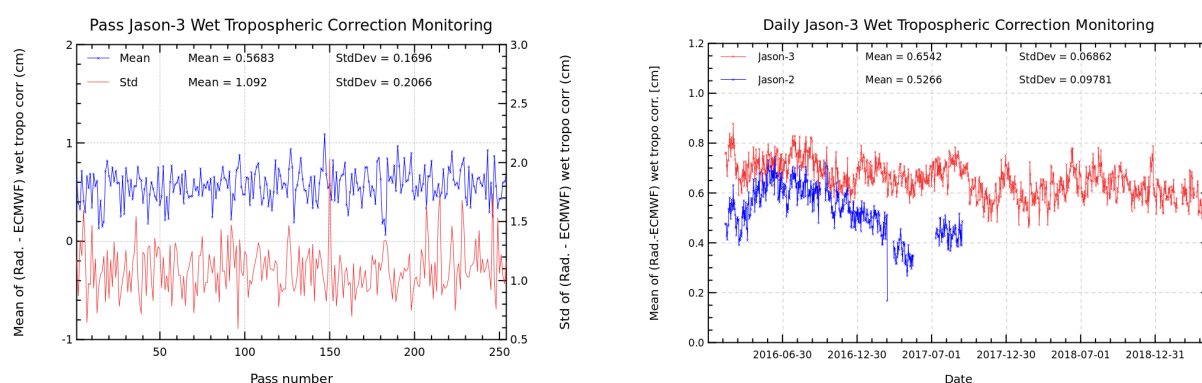
FIGURE 11 – Pass monitoring of wet troposphere differences between radiometer and ECMWF model for Jason-3 cycle 119 (left) and Jason-3 versus Jason-2 daily monitoring of wet troposphere differences between radiometer and ECMWF model (right).
