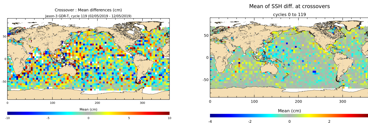
FIGURE 12 – Mean SSH at crossovers for cycle 119 (left) and over the whole Jason-3 period (right).
