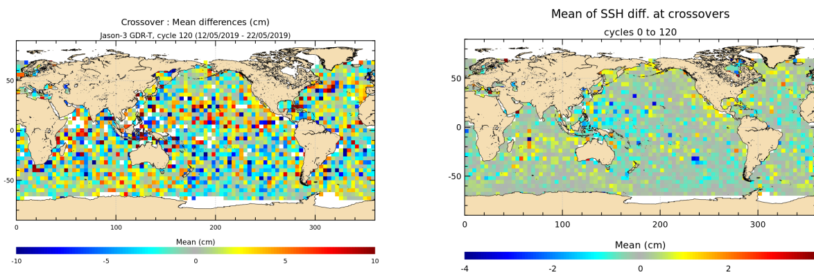
FIGURE 12 – Mean SSH at crossovers for cycle 120 (left) and over the whole Jason-3 period (right).
