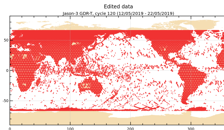
FIGURE 2 – Edited measurements for cycle 120.
