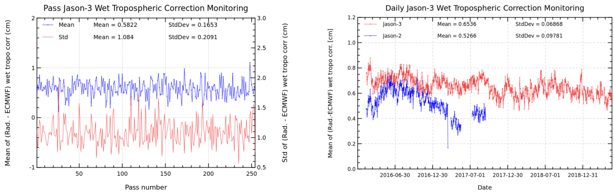
FIGURE 11 – Pass monitoring of wet troposphere differences between radiometer and ECMWF model for Jason-3 cycle 120 (left) and Jason-3 versus Jason-2 daily monitoring of wet troposphere differences between radiometer and ECMWF model (right).
