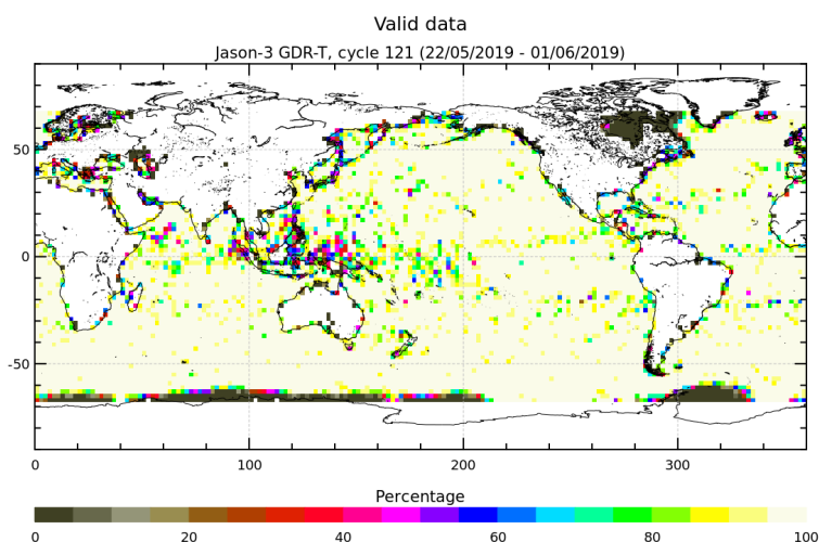
FIGURE 3 – Percentage of valid measurements for cycle 121.
