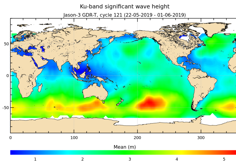
FIGURE 5 – Significant wave height for cycle 121.
