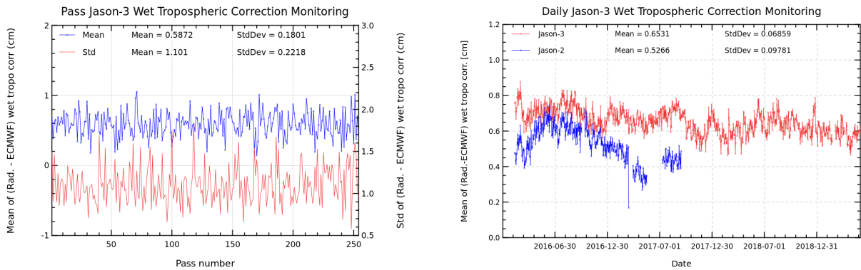
FIGURE 11 – Pass monitoring of wet troposphere differences between radiometer and ECMWF model for Jason-3 cycle 121 (left) and Jason-3 versus Jason-2 daily monitoring of wet troposphere differences between radiometer and ECMWF model (right).
