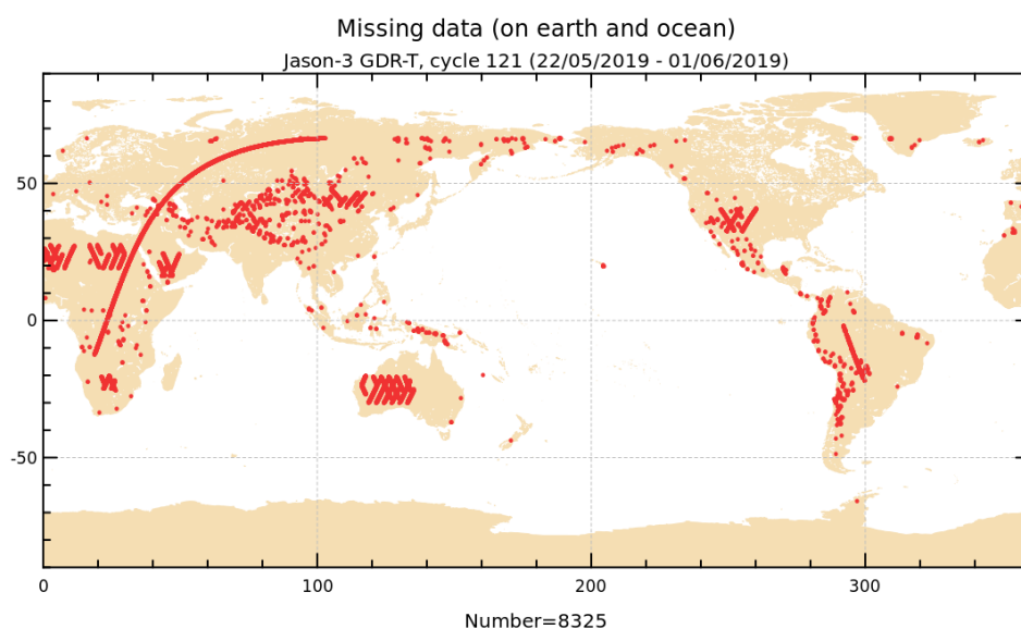
FIGURE 1 – Missing measurements for cycle 121.
