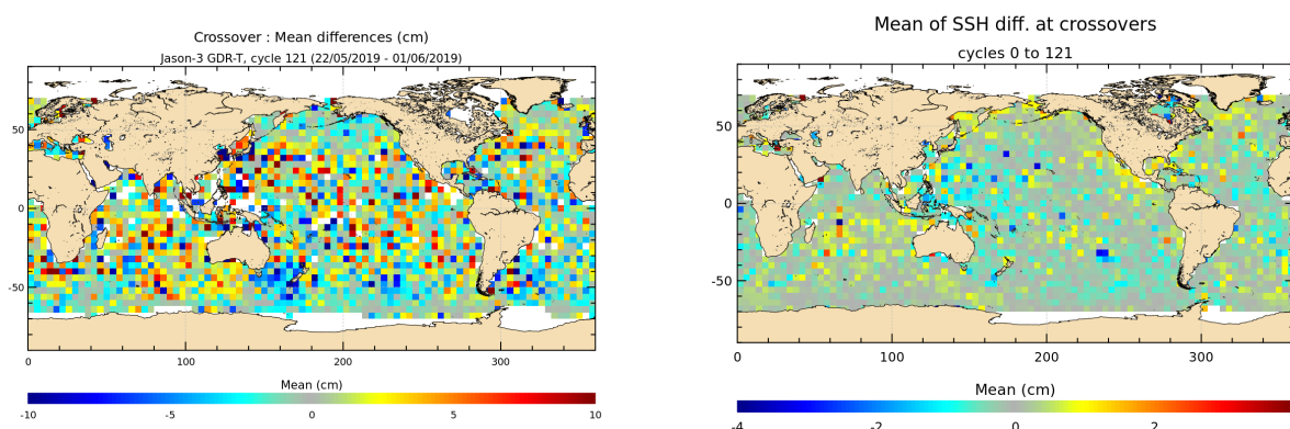
FIGURE 12 – Mean SSH at crossovers for cycle 121 (left) and over the whole Jason-3 period (right).
