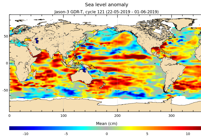
FIGURE 17 – Sea level anomaly relative to MSS for cycle 121.
