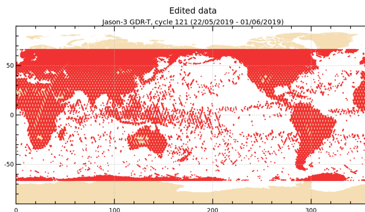
FIGURE 2 – Edited measurements for cycle 121.
