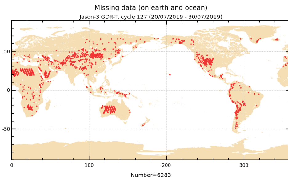
FIGURE 1 – Missing measurements for cycle 127.
