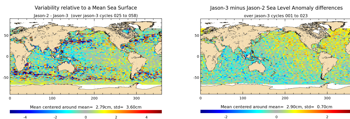
FIGURE 18 – Jason-2 – Jason-3 SLA differences averaged over Jason-3 period from cycle 025 until cycle 058 (left), and for tandem phase (cycle 001 to 023) (right).
