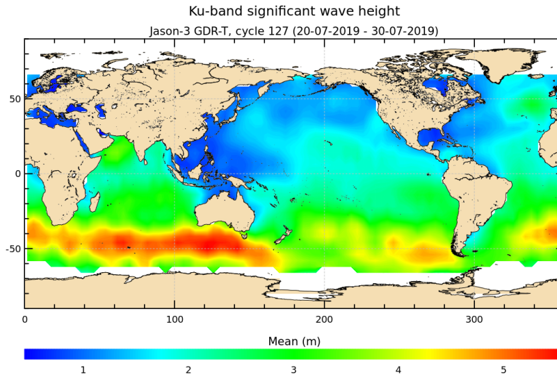
FIGURE 5 – Significant wave height for cycle 127.
