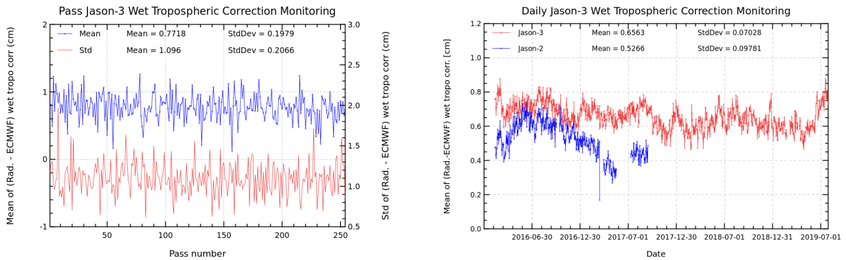
FIGURE 11 – Pass monitoring of wet troposphere differences between radiometer and ECMWF model for Jason-3 cycle 127 (left) and Jason-3 versus Jason-2 daily monitoring of wet troposphere differences between radiometer and ECMWF model (right).
