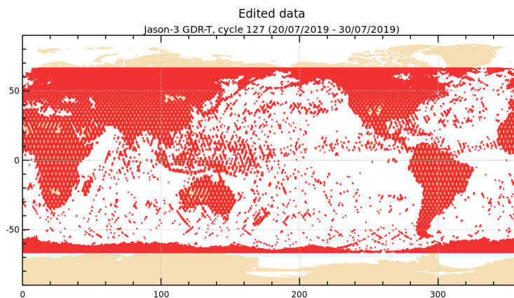
FIGURE 2 – Edited measurements for cycle 127.
