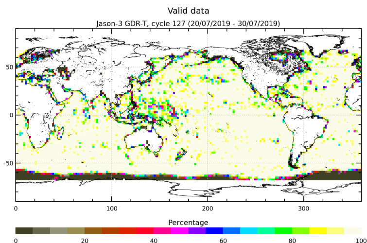
FIGURE 3 – Percentage of valid measurements for cycle 127.
