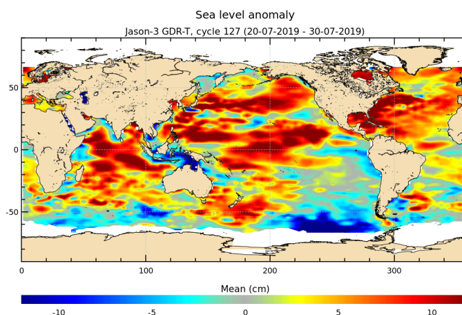
FIGURE 17 – Sea level anomaly relative to MSS for cycle 127.
