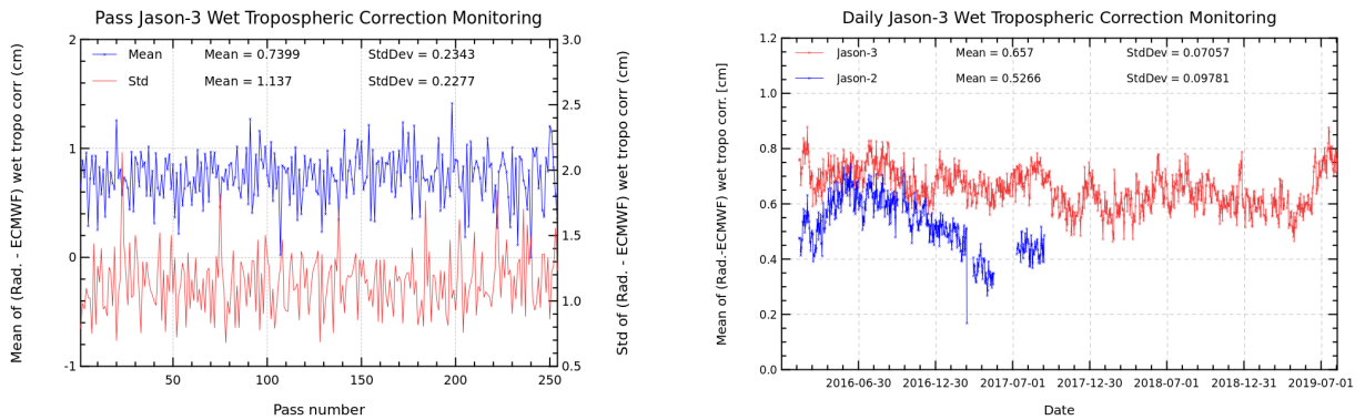
FIGURE 11 – Pass monitoring of wet troposphere differences between radiometer and ECMWF model for Jason-3 cycle 128 (left) and Jason-3 versus Jason-2 daily monitoring of wet troposphere differences between radiometer and ECMWF model (right).
