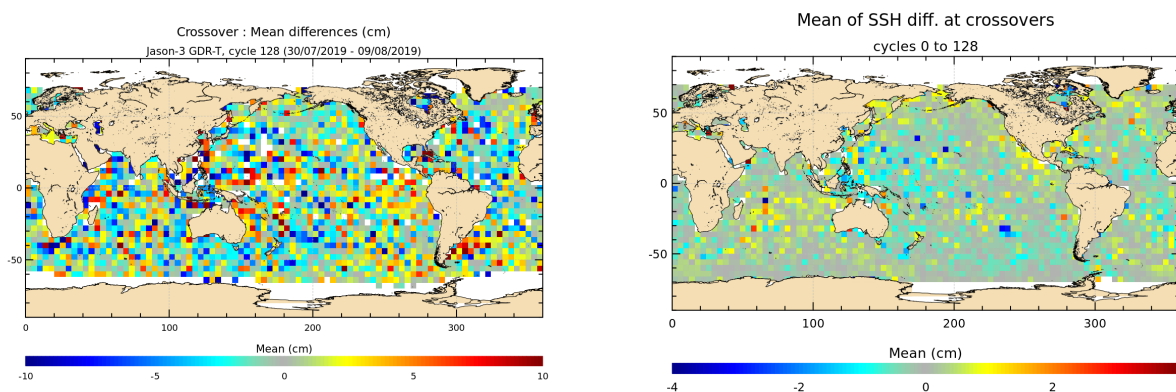
FIGURE 12 – Mean SSH at crossovers for cycle 128 (left) and over the whole Jason-3 period (right).
