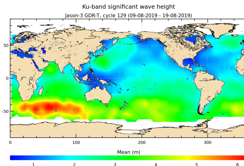
FIGURE 5 – Significant wave height for cycle 129.
