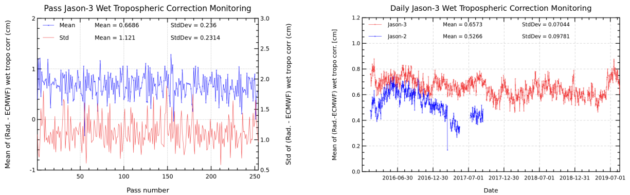
FIGURE 11 – Pass monitoring of wet troposphere differences between radiometer and ECMWF model for Jason-3 cycle 129 (left) and Jason-3 versus Jason-2 daily monitoring of wet troposphere differences between radiometer and ECMWF model (right).
