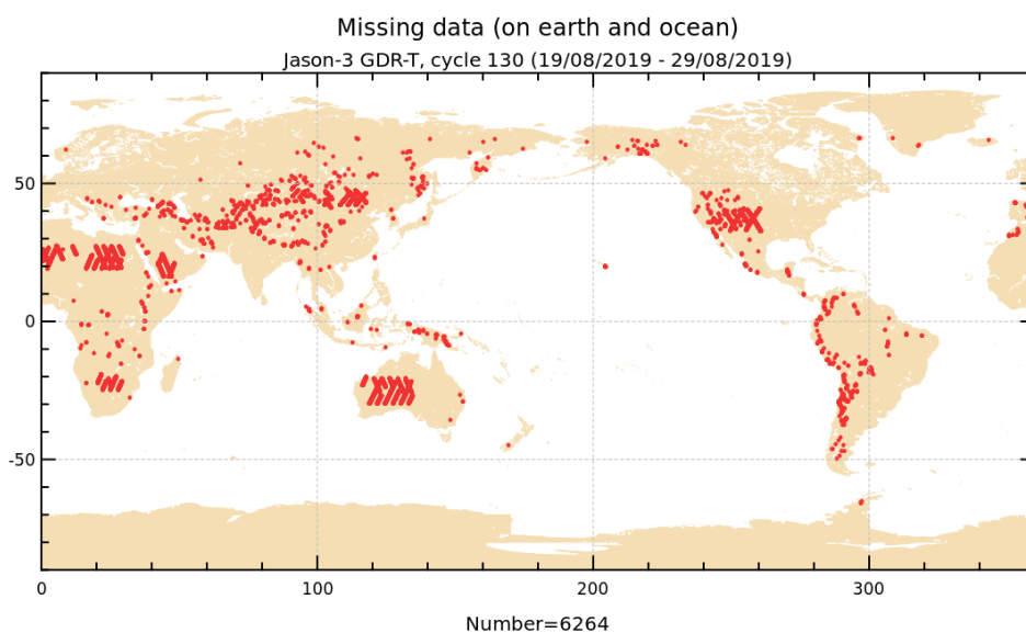
FIGURE 1 – Missing measurements for cycle 130.
