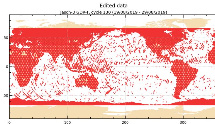
FIGURE 2 – Edited measurements for cycle 130.
