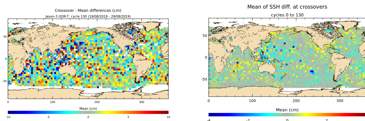
FIGURE 12 – Mean SSH at crossovers for cycle 130 (left) and over the whole Jason-3 period (right).
