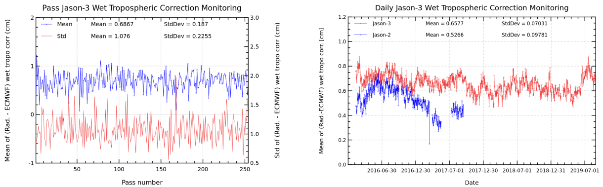
FIGURE 11 – Pass monitoring of wet troposphere differences between radiometer and ECMWF model for Jason-3 cycle 130 (left) and Jason-3 versus Jason-2 daily monitoring of wet troposphere differences between radiometer and ECMWF model (right).
