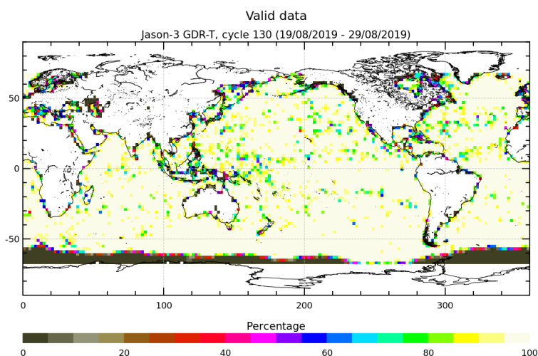
FIGURE 3 – Percentage of valid measurements for cycle 130.
