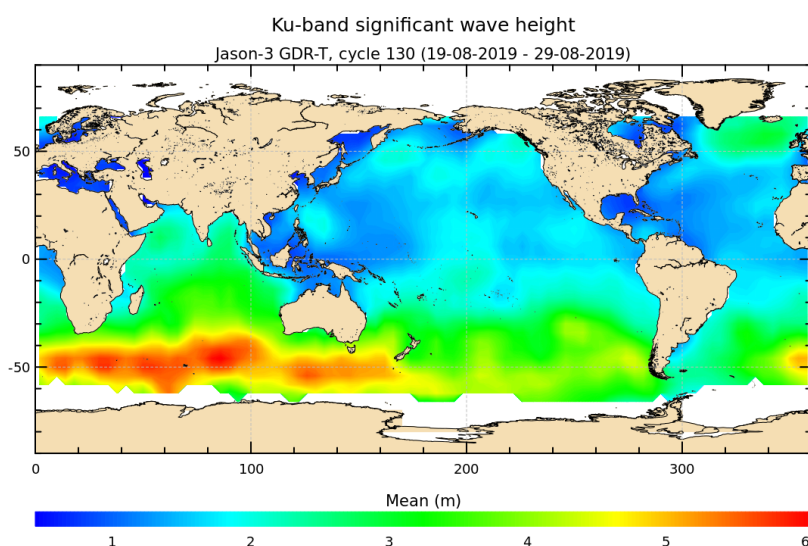
FIGURE 5 – Significant wave height for cycle 130.
