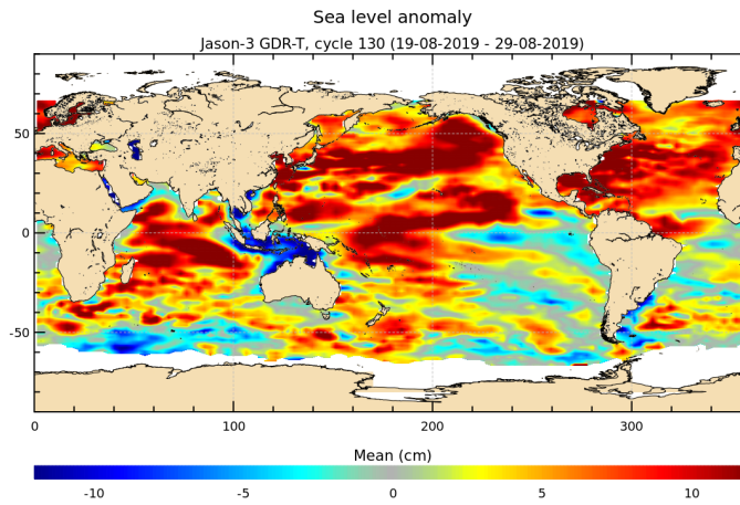
FIGURE 17 – Sea level anomaly relative to MSS for cycle 130.
