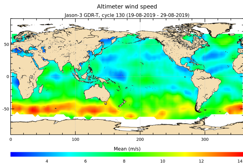
FIGURE 9 – Altimeter wind speed for cycle 130.
