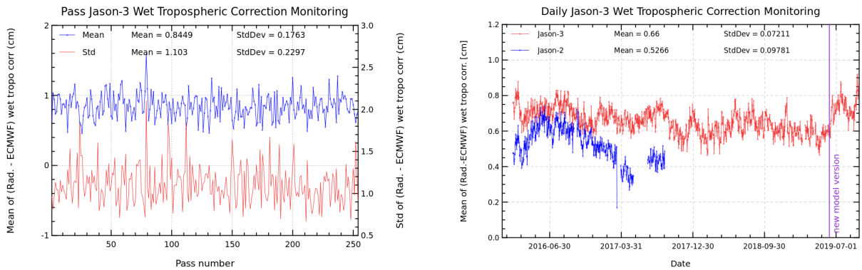
FIGURE 11 – Pass monitoring of wet troposphere differences between radiometer and ECMWF model for Jason-3 cycle 133 (left) and Jason-3 versus Jason-2 daily monitoring of wet troposphere differences between radiometer and ECMWF model (right).
