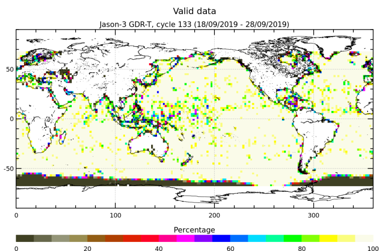
FIGURE 3 – Percentage of valid measurements for cycle 133.
