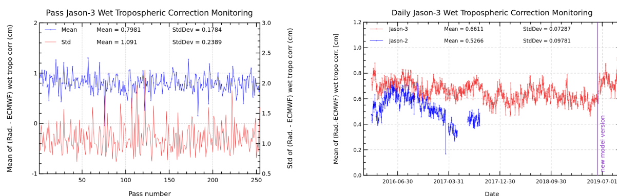
FIGURE 11 – Pass monitoring of wet troposphere differences between radiometer and ECMWF model for Jason-3 cycle 134 (left) and Jason-3 versus Jason-2 daily monitoring of wet troposphere differences between radiometer and ECMWF model (right).
