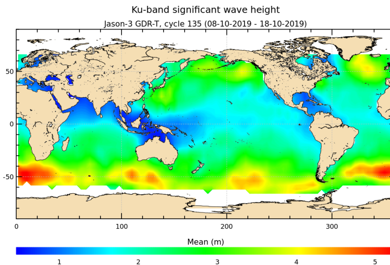
FIGURE 5 – Significant wave height for cycle 135.
