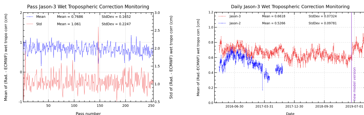
FIGURE 11 – Pass monitoring of wet troposphere differences between radiometer and ECMWF model for Jason-3 cycle 135 (left) and Jason-3 versus Jason-2 daily monitoring of wet troposphere differences between radiometer and ECMWF model (right).
