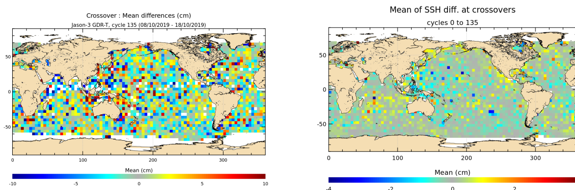
FIGURE 12 – Mean SSH at crossovers for cycle 135 (left) and over the whole Jason-3 period (right).
