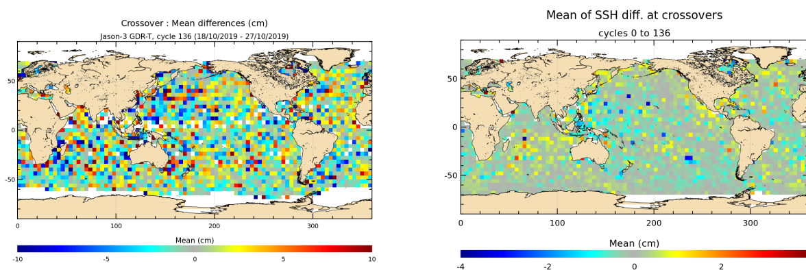
FIGURE 12 – Mean SSH at crossovers for cycle 136 (left) and over the whole Jason-3 period (right).
