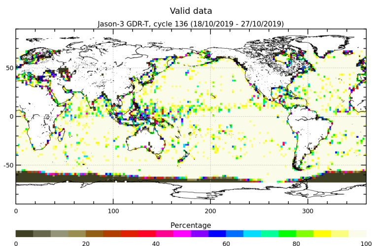
FIGURE 3 – Percentage of valid measurements for cycle 136.
