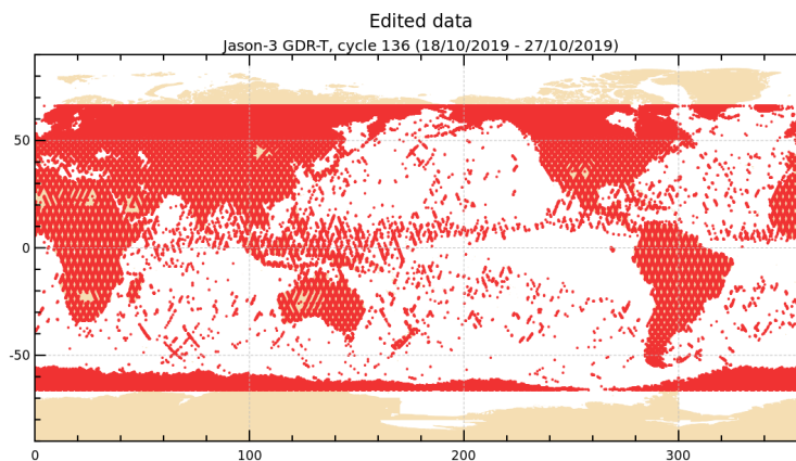
FIGURE 2 – Edited measurements for cycle 136.
