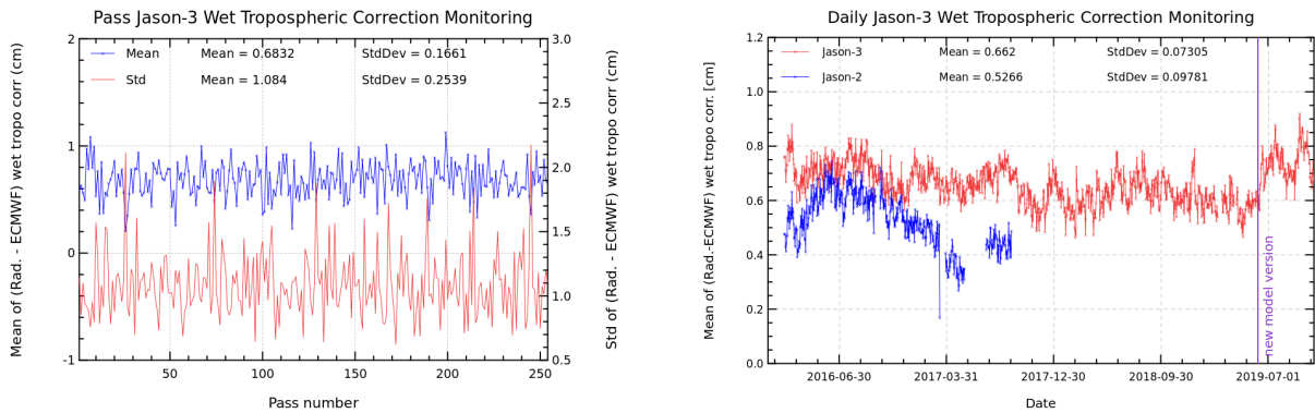
FIGURE 11 – Pass monitoring of wet troposphere differences between radiometer and ECMWF model for Jason-3 cycle 136 (left) and Jason-3 versus Jason-2 daily monitoring of wet troposphere differences between radiometer and ECMWF model (right).
