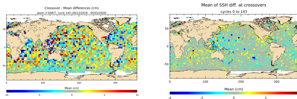
FIGURE 12 – Mean SSH at crossovers for cycle 143 (left) and over the whole Jason-3 period (right).
