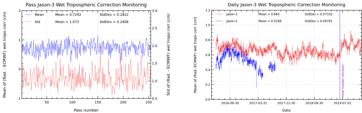
FIGURE 11 – Pass monitoring of wet troposphere differences between radiometer and ECMWF model for Jason-3 cycle 143 (left) and Jason-3 versus Jason-2 daily monitoring of wet troposphere differences between radiometer and ECMWF model (right).
