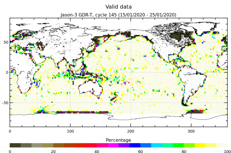
FIGURE 3 – Percentage of valid measurements for cycle 145.
