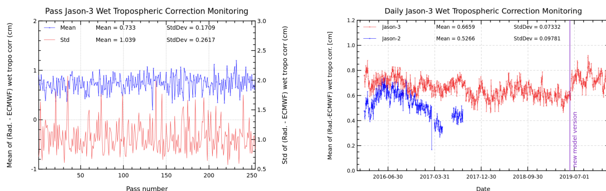
FIGURE 11 – Pass monitoring of wet troposphere differences between radiometer and ECMWF model for Jason-3 cycle 145 (left) and Jason-3 versus Jason-2 daily monitoring of wet troposphere differences between radiometer and ECMWF model (right).
