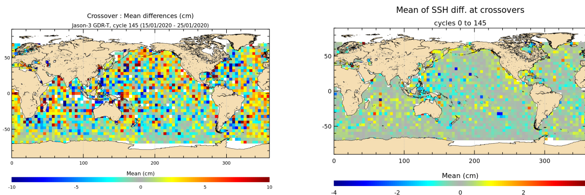
FIGURE 13 – Mean SSH at crossovers for cycle 145 (left) and over the whole Jason-3 period (right).
