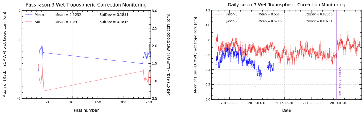
FIGURE 12 – Pass monitoring of wet troposphere differences between radiometer and ECMWF model for Jason-3 cycle 147 (left) and Jason-3 versus Jason-2 daily monitoring of wet troposphere differences between radiometer and ECMWF model (right).
