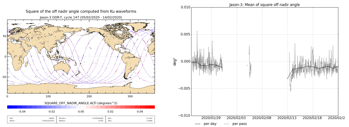
FIGURE 4 – Map and daily monitoring of apparent squared mispointing from waveforms for cycle 147.
