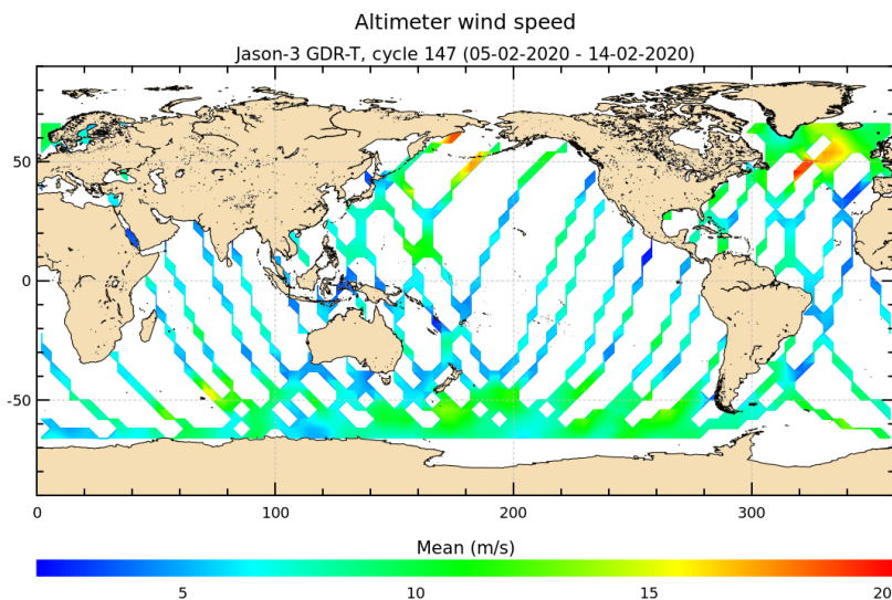
FIGURE 10 – Altimeter wind speed for cycle 147.
