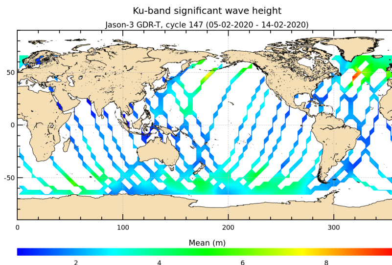
FIGURE 6 – Significant wave height for cycle 147.
