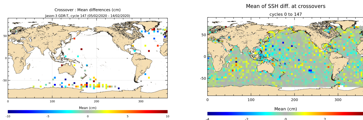
FIGURE 13 – Mean SSH at crossovers for cycle 147 (left) and over the whole Jason-3 period (right).
