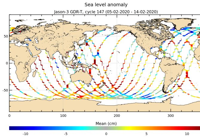
FIGURE 18 – Sea level anomaly relative to MSS for cycle 147.
