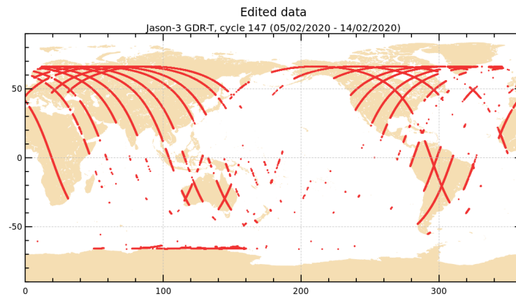
FIGURE 2 – Edited measurements for cycle 147.
