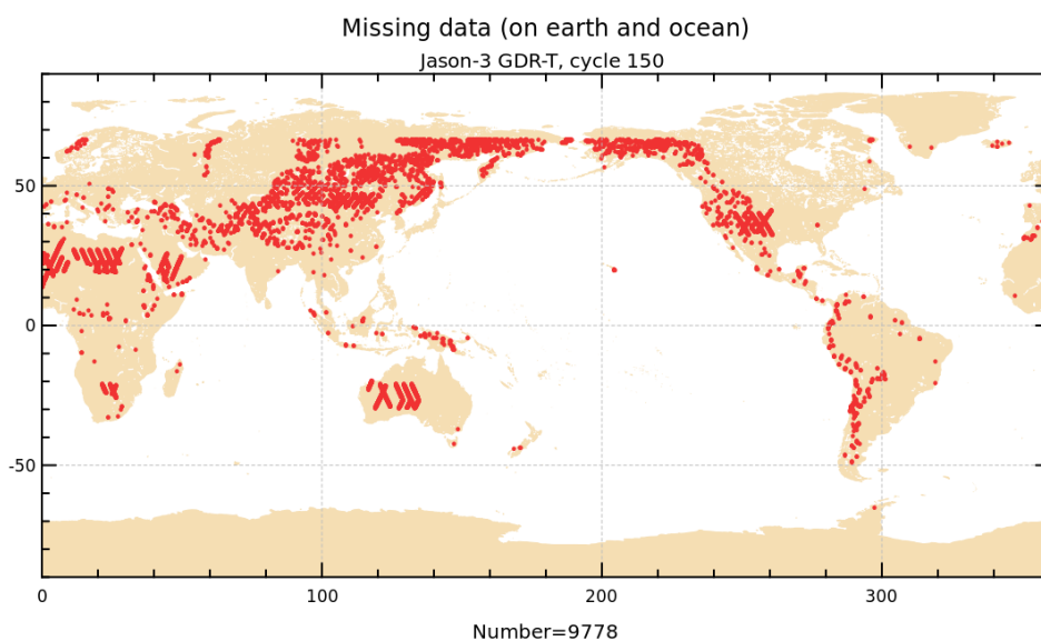
FIGURE 1 – Missing measurements for cycle 150.
