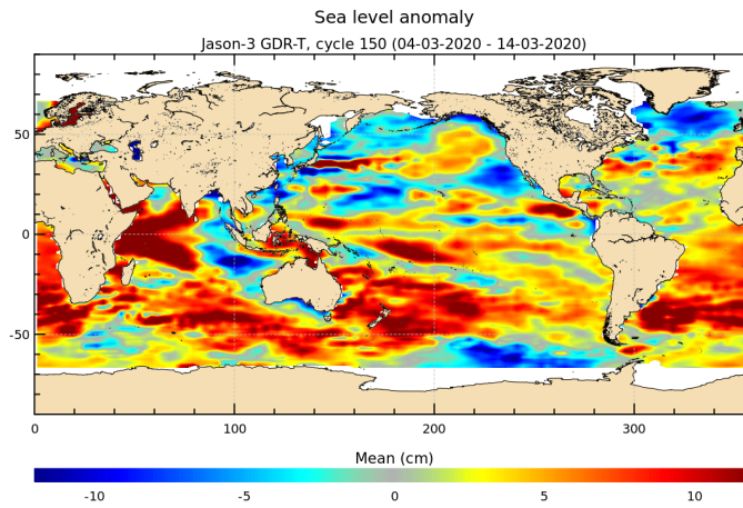
FIGURE 17 – Sea level anomaly relative to MSS for cycle 150.
