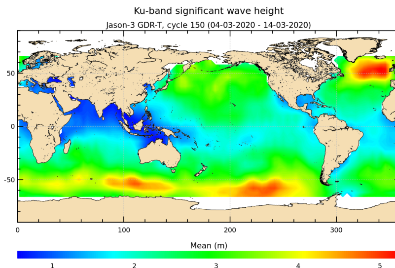
FIGURE 5 – Significant wave height for cycle 150.
