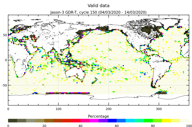
FIGURE 3 – Percentage of valid measurements for cycle 150.
