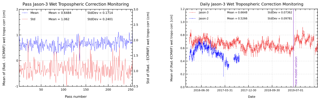
FIGURE 11 – Pass monitoring of wet troposphere differences between radiometer and ECMWF model for Jason-3 cycle 150 (left) and Jason-3 versus Jason-2 daily monitoring of wet troposphere differences between radiometer and ECMWF model (right).
