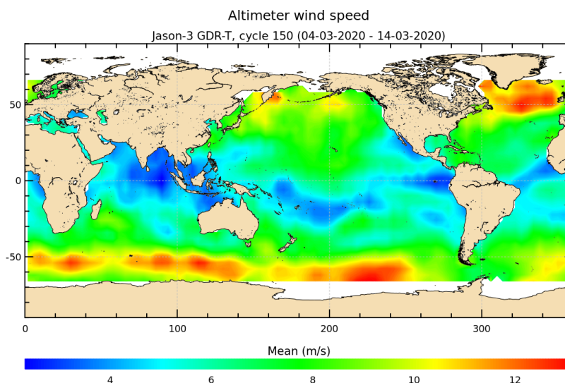
FIGURE 9 – Altimeter wind speed for cycle 150.
