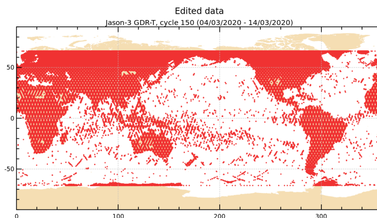
FIGURE 2 – Edited measurements for cycle 150.
