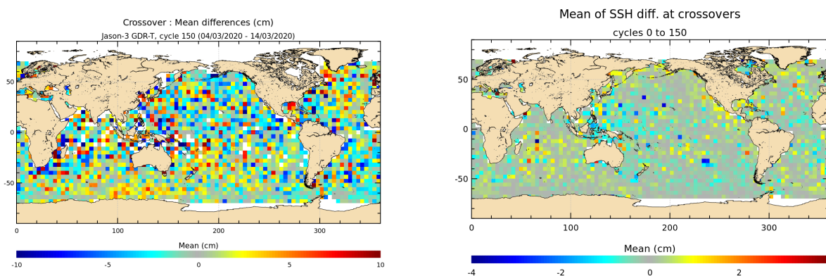
FIGURE 12 – Mean SSH at crossovers for cycle 150 (left) and over the whole Jason-3 period (right).
