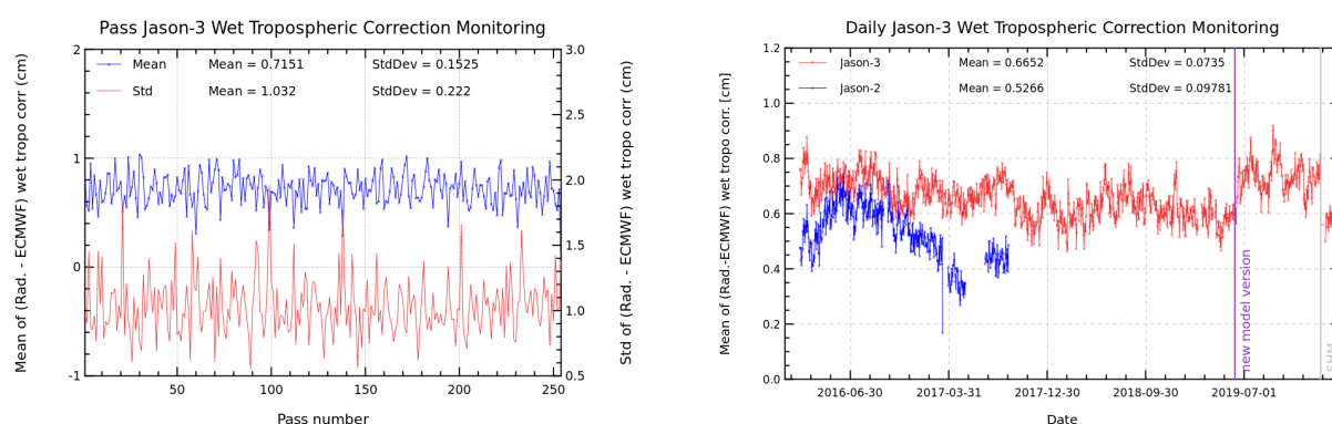
FIGURE 11 – Pass monitoring of wet troposphere differences between radiometer and ECMWF model for Jason-3 cycle 151 (left) and Jason-3 versus Jason-2 daily monitoring of wet troposphere differences between radiometer and ECMWF model (right).
