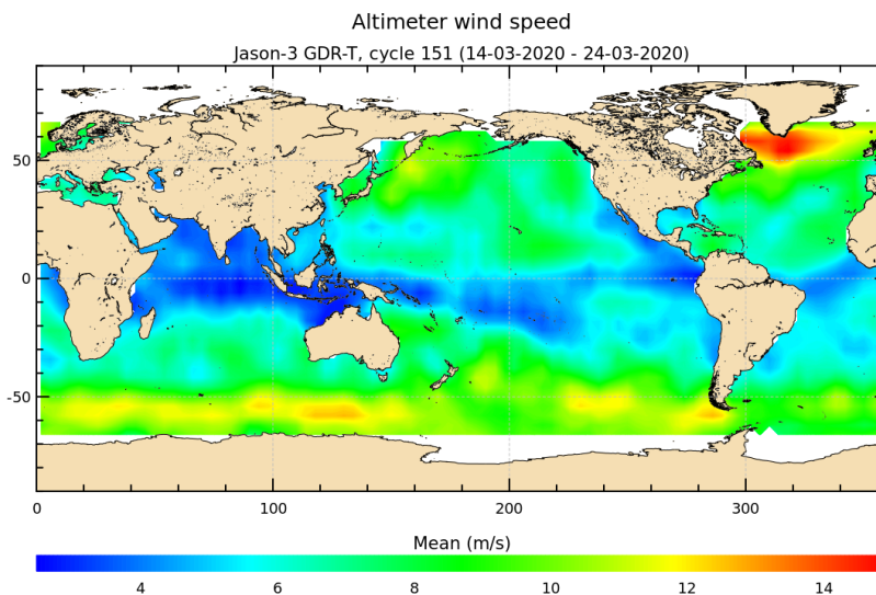
FIGURE 9 – Altimeter wind speed for cycle 151.
