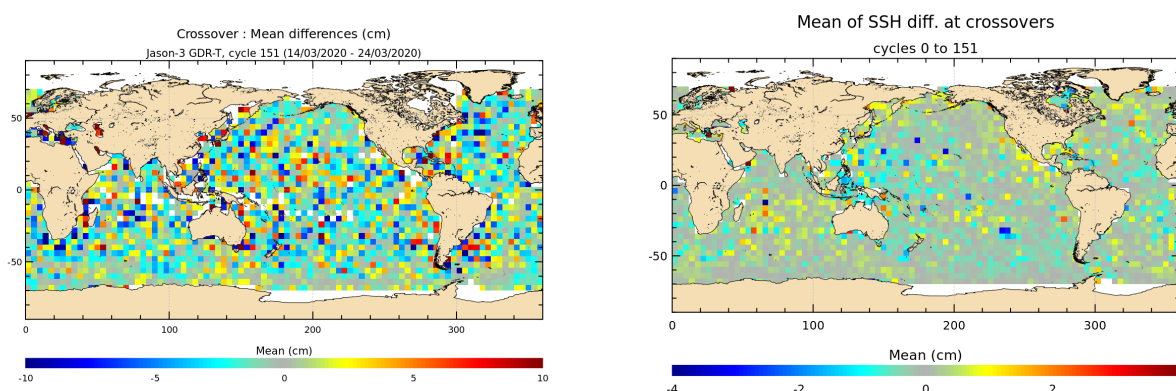
FIGURE 12 – Mean SSH at crossovers for cycle 151 (left) and over the whole Jason-3 period (right).
