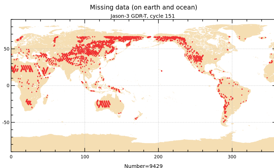
FIGURE 1 – Missing measurements for cycle 151.
