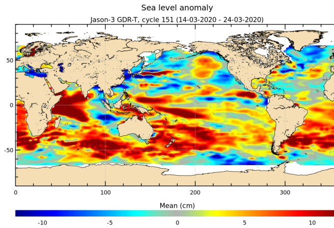
FIGURE 17 – Sea level anomaly relative to MSS for cycle 151.
