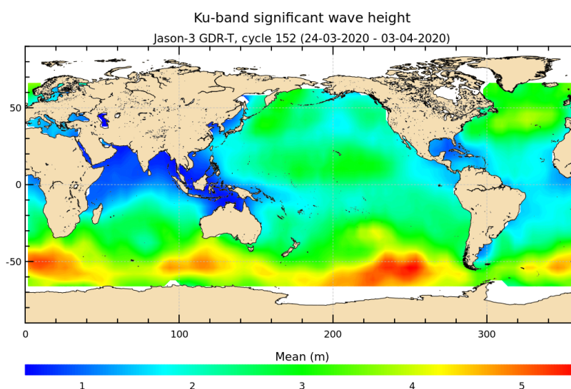
FIGURE 5 – Significant wave height for cycle 152.
