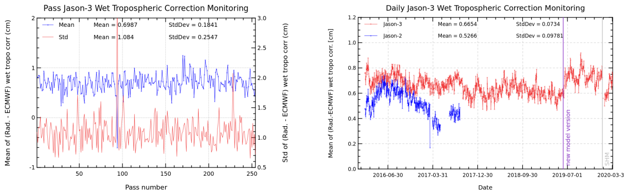
FIGURE 11 – Pass monitoring of wet troposphere differences between radiometer and ECMWF model for Jason-3 cycle 152 (left) and Jason-3 versus Jason-2 daily monitoring of wet troposphere differences between radiometer and ECMWF model (right).
