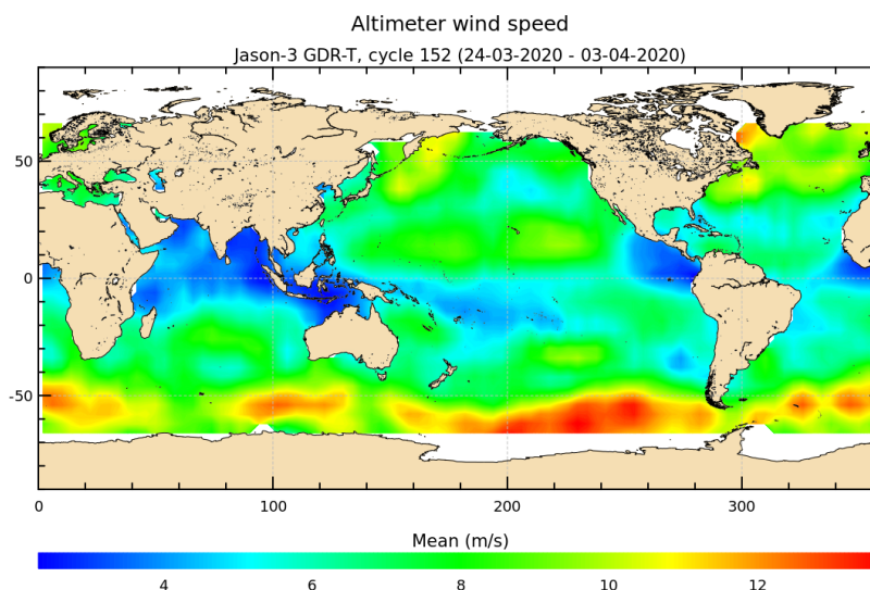
FIGURE 9 – Altimeter wind speed for cycle 152.
