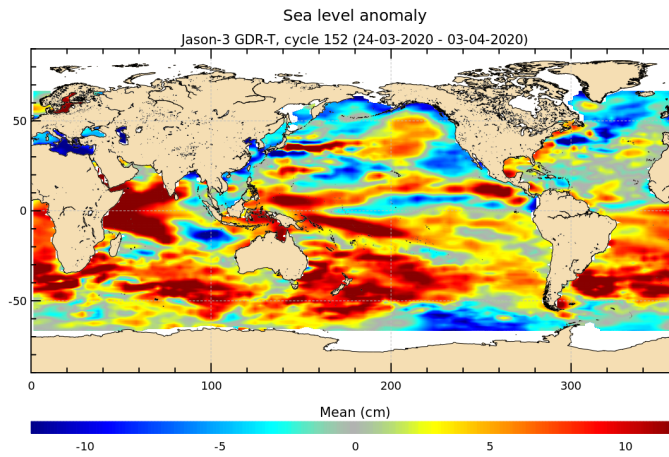
FIGURE 17 – Sea level anomaly relative to MSS for cycle 152.
