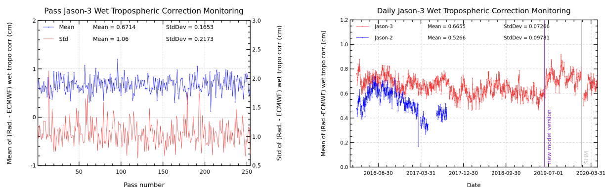
FIGURE 11 – Pass monitoring of wet troposphere differences between radiometer and ECMWF model for Jason-3 cycle 156 (left) and Jason-3 versus Jason-2 daily monitoring of wet troposphere differences between radiometer and ECMWF model (right).
