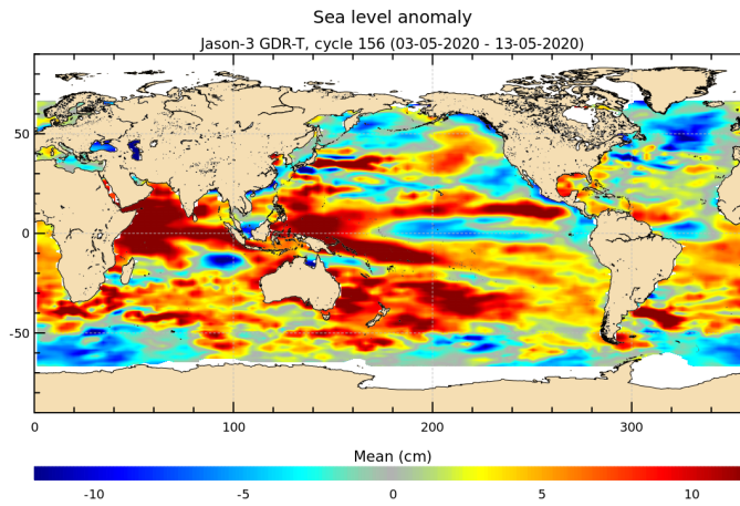
FIGURE 17 – Sea level anomaly relative to MSS for cycle 156.
