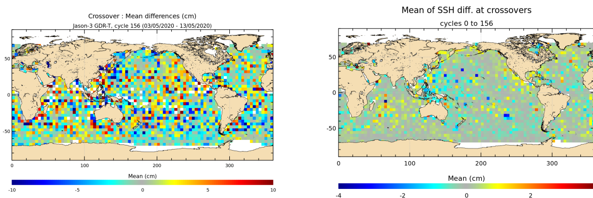
FIGURE 12 – Mean SSH at crossovers for cycle 156 (left) and over the whole Jason-3 period (right).
