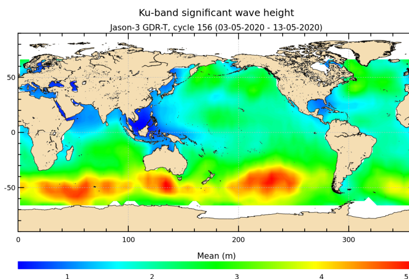
FIGURE 5 – Significant wave height for cycle 156.
