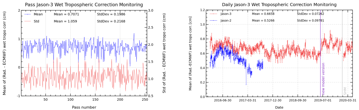
FIGURE 11 – Pass monitoring of wet troposphere differences between radiometer and ECMWF model for Jason-3 cycle 157 (left) and Jason-3 versus Jason-2 daily monitoring of wet troposphere differences between radiometer and ECMWF model (right).
