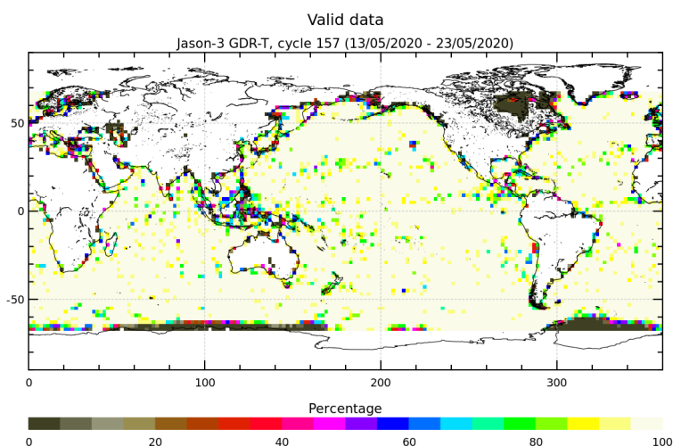
FIGURE 3 – Percentage of valid measurements for cycle 157.
