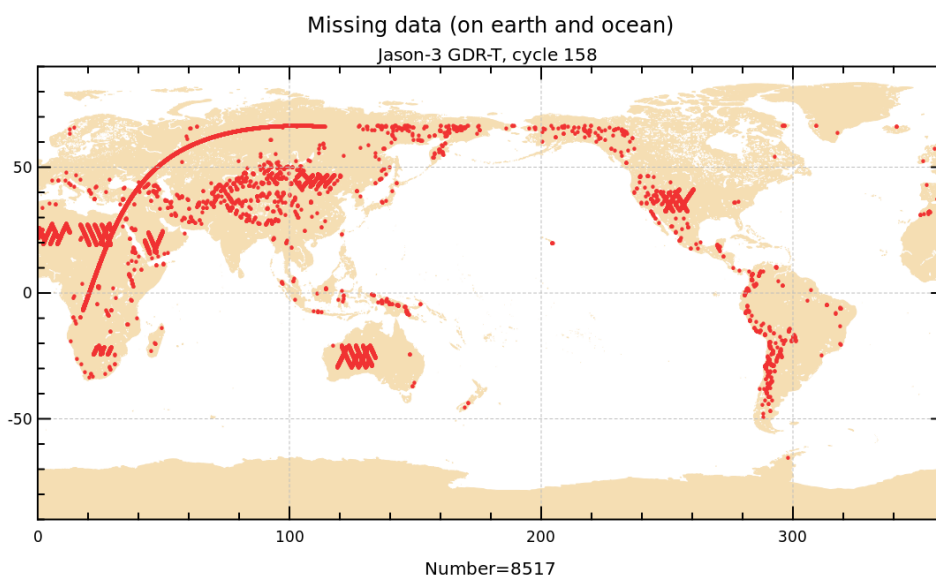
FIGURE 1 – Missing measurements for cycle 158.
