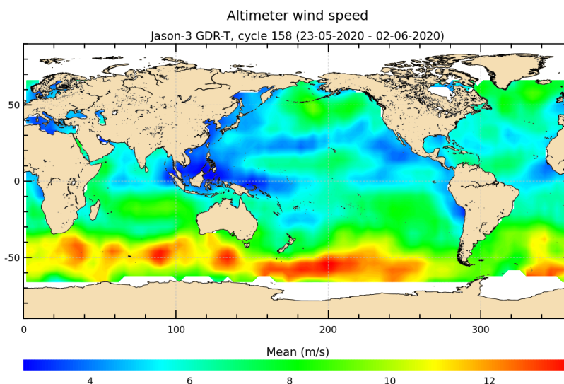
FIGURE 9 – Altimeter wind speed for cycle 158.
