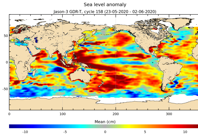
FIGURE 17 – Sea level anomaly relative to MSS for cycle 158.
