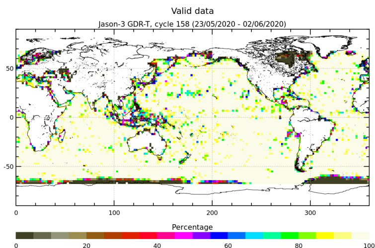
FIGURE 3 – Percentage of valid measurements for cycle 158.
