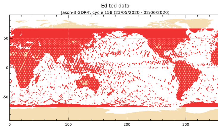
FIGURE 2 – Edited measurements for cycle 158.
