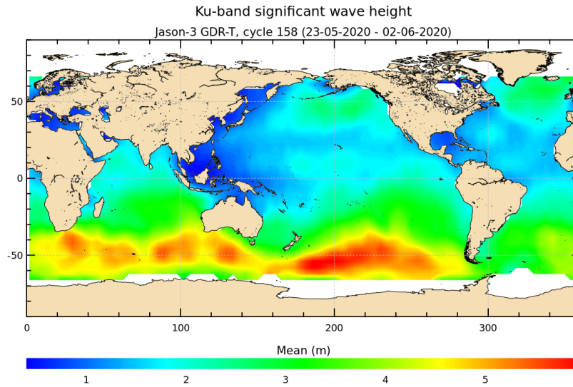
FIGURE 5 – Significant wave height for cycle 158.
