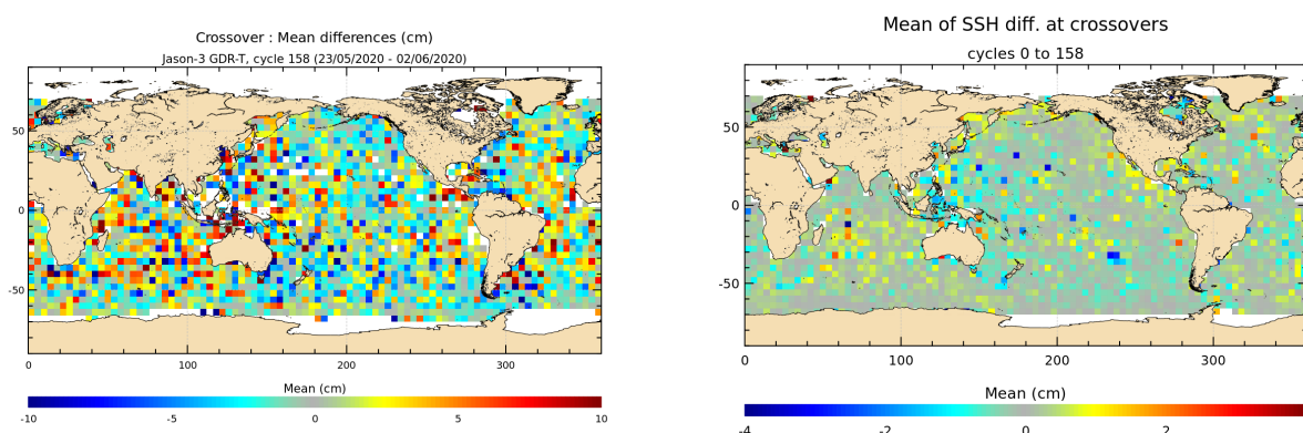
FIGURE 12 – Mean SSH at crossovers for cycle 158 (left) and over the whole Jason-3 period (right).
