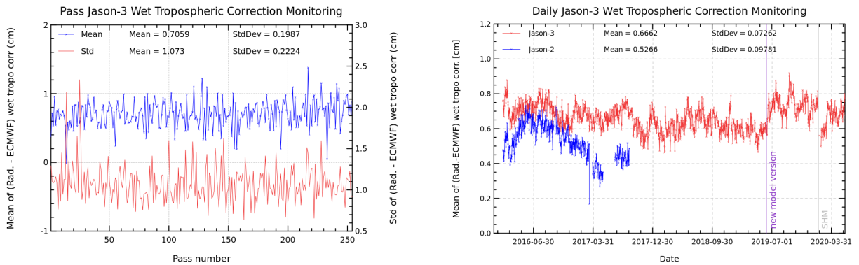
FIGURE 11 – Pass monitoring of wet troposphere differences between radiometer and ECMWF model for Jason-3 cycle 158 (left) and Jason-3 versus Jason-2 daily monitoring of wet troposphere differences between radiometer and ECMWF model (right).
