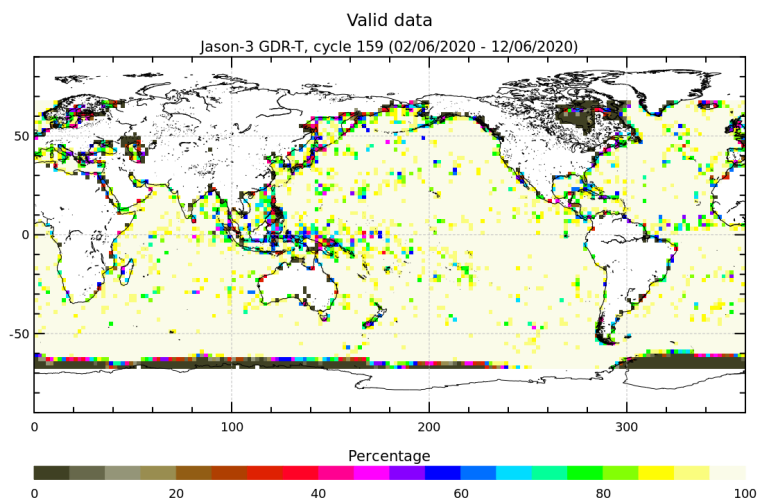
FIGURE 3 – Percentage of valid measurements for cycle 159.
