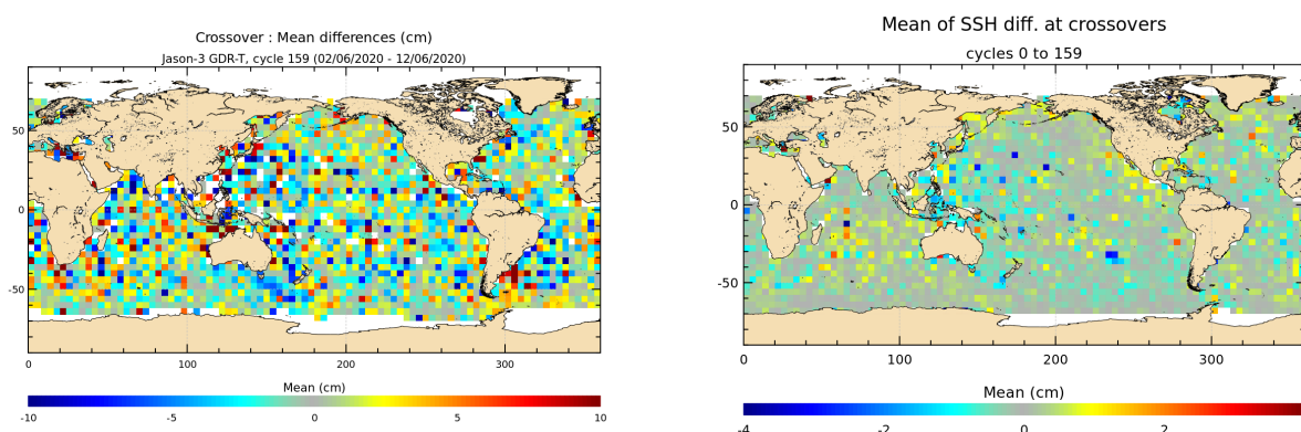
FIGURE 12 – Mean SSH at crossovers for cycle 159 (left) and over the whole Jason-3 period (right).
