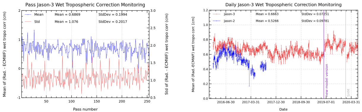
FIGURE 11 – Pass monitoring of wet troposphere differences between radiometer and ECMWF model for Jason-3 cycle 159 (left) and Jason-3 versus Jason-2 daily monitoring of wet troposphere differences between radiometer and ECMWF model (right).
